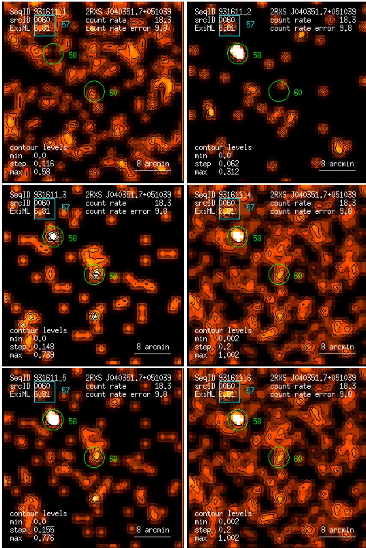
Figure 60: RASS 931611: detection 0060: band rate images, Gaussian filter: (1) PSPC channels 11 – 41, (2) 52 – 90, (3) 91 – 201, (4) 11 – 235, (5) 52 – 201, (6) 11 – 201. Broad band rates in counts/ks. Band rate contour levels in counts/ks/arcmin 2 .
