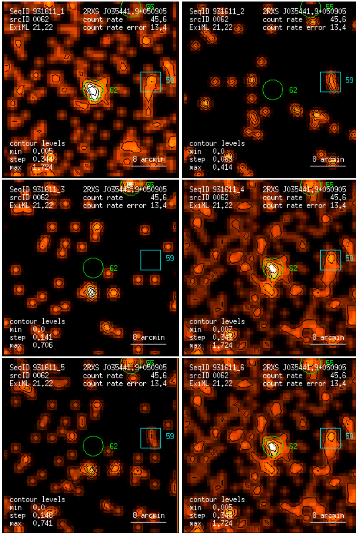
Figure 62: RASS 931611: detection 0062: band rate images, Gaussian filter: (1) PSPC channels 11 – 41, (2) 52 – 90, (3) 91 – 201, (4) 11 – 235, (5) 52 – 201, (6) 11 – 201. Broad band rates in counts/ks. Band rate contour levels in counts/ks/arcmin 2 .
