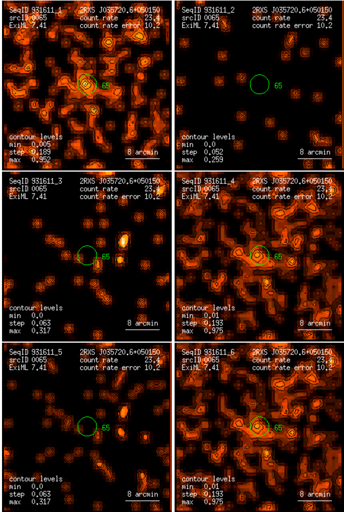
Figure 65: RASS 931611: detection 0065: band rate images, Gaussian filter: (1) PSPC channels 11 – 41, (2) 52 – 90, (3) 91 – 201, (4) 11 – 235, (5) 52 – 201, (6) 11 – 201. Broad band rates in counts/ks. Band rate contour levels in counts/ks/arcmin 2 .
