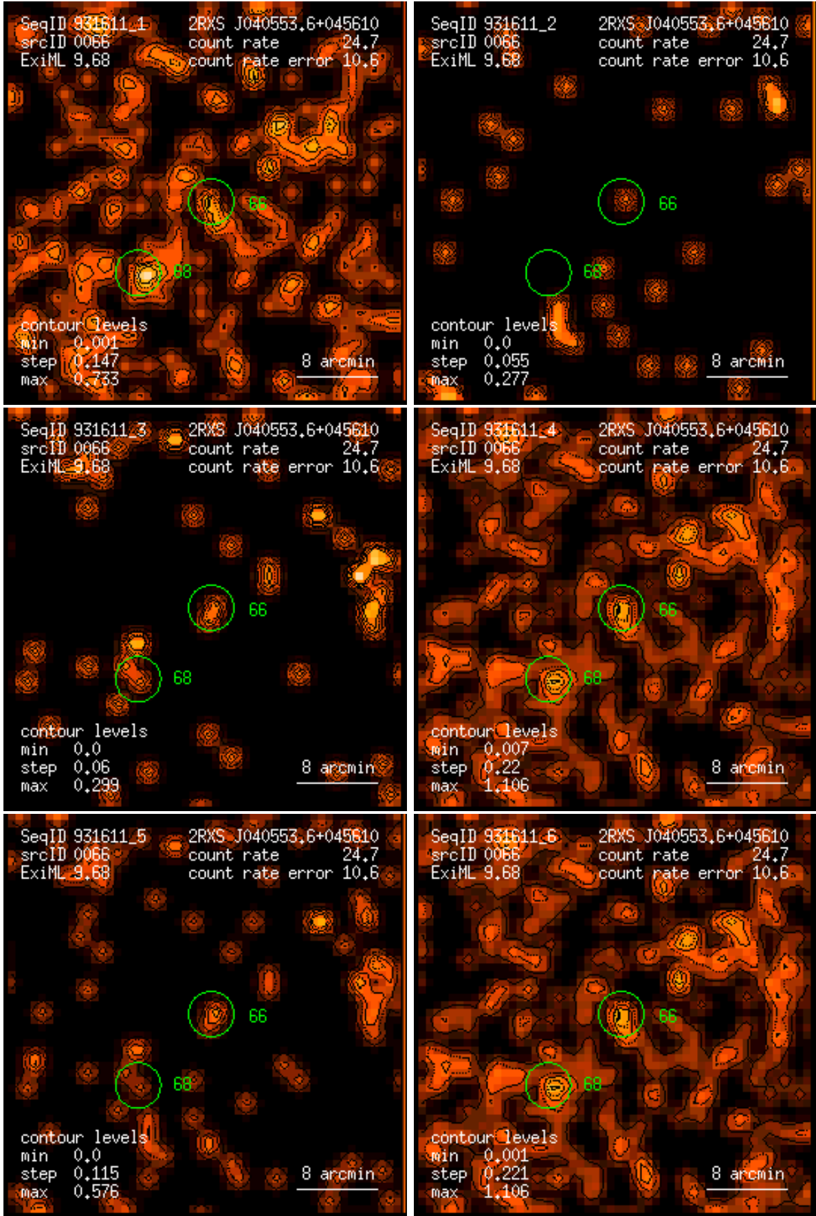
Figure 66: RASS 931611: detection 0066: band rate images, Gaussian filter: (1) PSPC channels 11 – 41, (2) 52 – 90, (3) 91 – 201, (4) 11 – 235, (5) 52 – 201, (6) 11 – 201. Broad band rates in counts/ks. Band rate contour levels in counts/ks/arcmin 2 .
