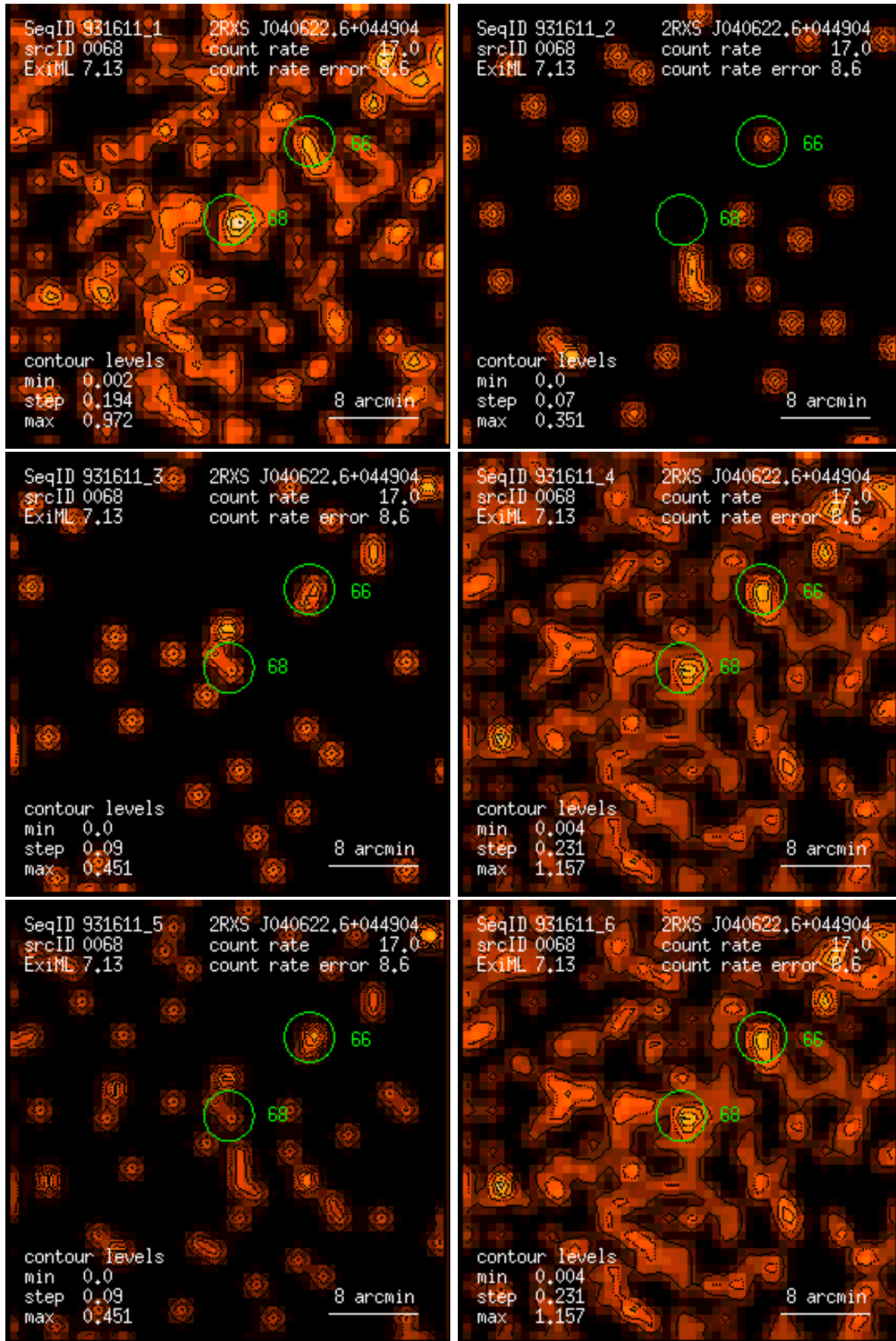
Figure 68: RASS 931611: detection 0068: band rate images, Gaussian filter: (1) PSPC channels 11 – 41, (2) 52 – 90, (3) 91 – 201, (4) 11 – 235, (5) 52 – 201, (6) 11 – 201. Broad band rates in counts/ks. Band rate contour levels in counts/ks/arcmin 2 .
