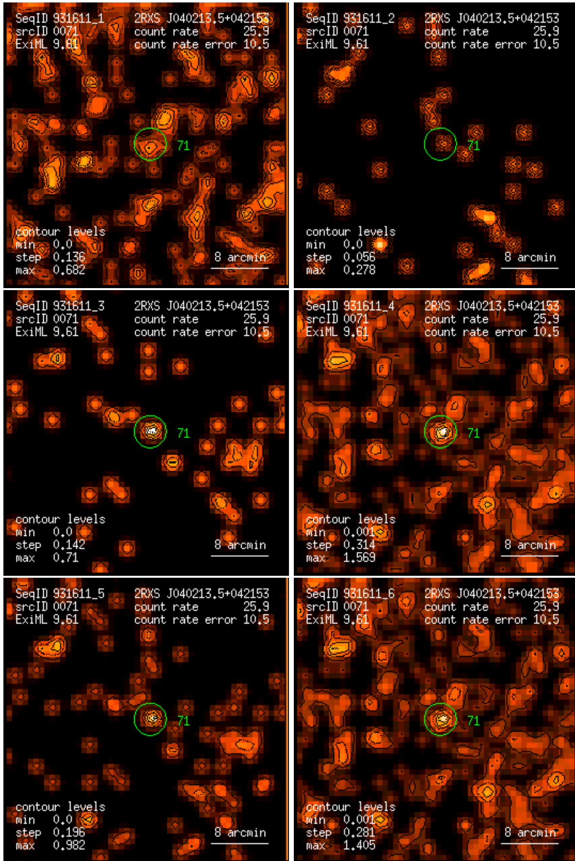
Figure 71: RASS 931611: detection 0071: band rate images, Gaussian filter: (1) PSPC channels 11 – 41, (2) 52 – 90, (3) 91 – 201, (4) 11 – 235, (5) 52 – 201, (6) 11 – 201. Broad band rates in counts/ks. Band rate contour levels in counts/ks/arcmin 2 .
