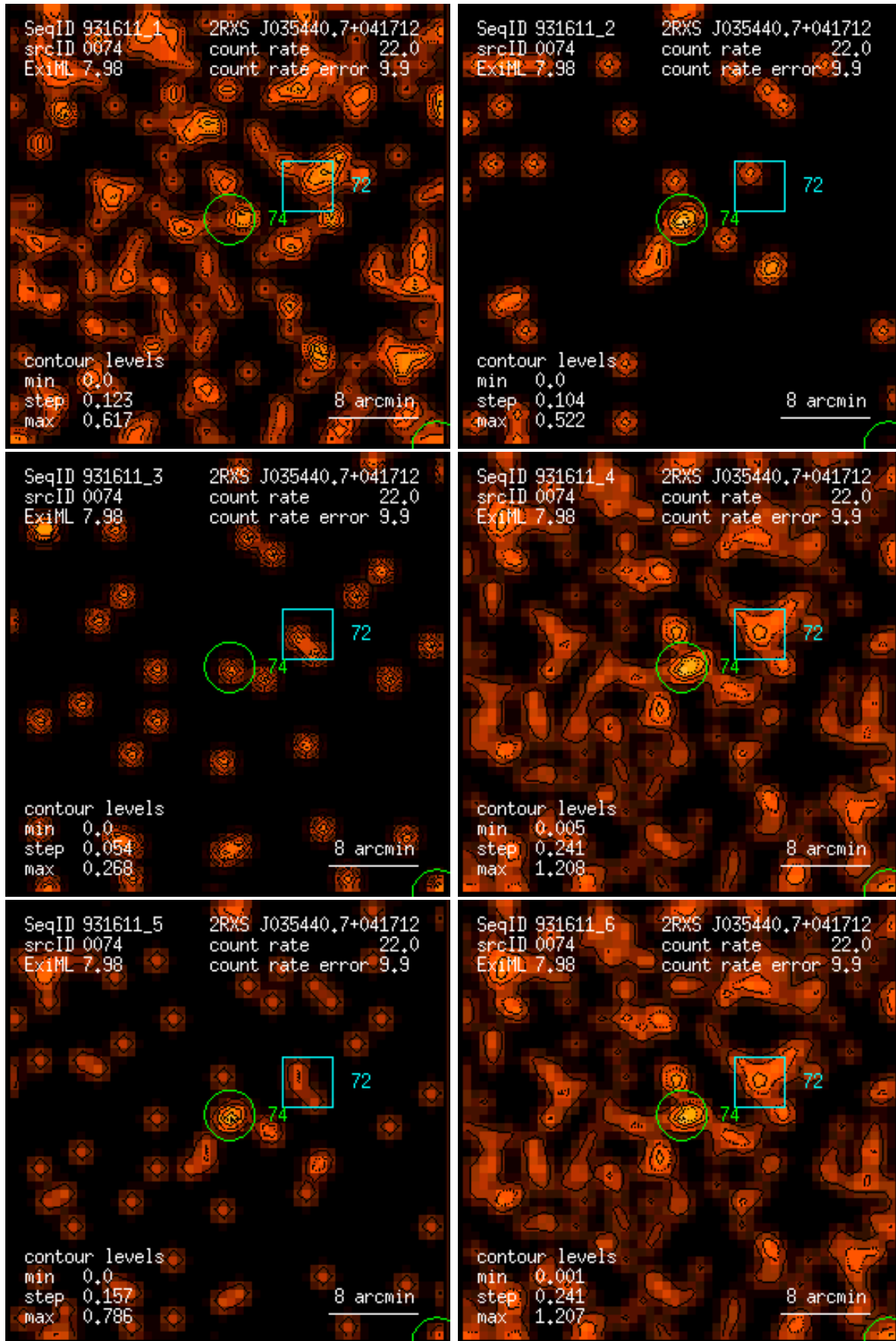
Figure 74: RASS 931611: detection 0074: band rate images, Gaussian filter: (1) PSPC channels 11 – 41, (2) 52 – 90, (3) 91 – 201, (4) 11 – 235, (5) 52 – 201, (6) 11 – 201. Broad band rates in counts/ks. Band rate contour levels in counts/ks/arcmin 2 .
