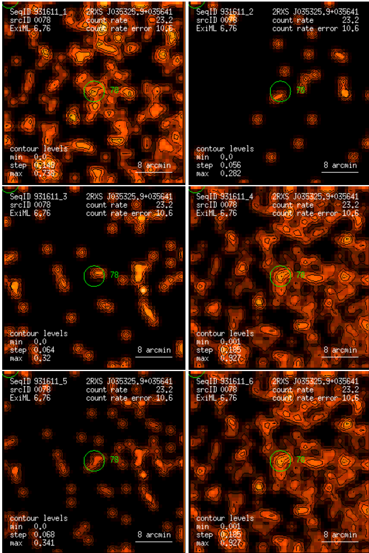
Figure 78: RASS 931611: detection 0078: band rate images, Gaussian filter: (1) PSPC channels 11 – 41, (2) 52 – 90, (3) 91 – 201, (4) 11 – 235, (5) 52 – 201, (6) 11 – 201. Broad band rates in counts/ks. Band rate contour levels in counts/ks/arcmin 2 .
