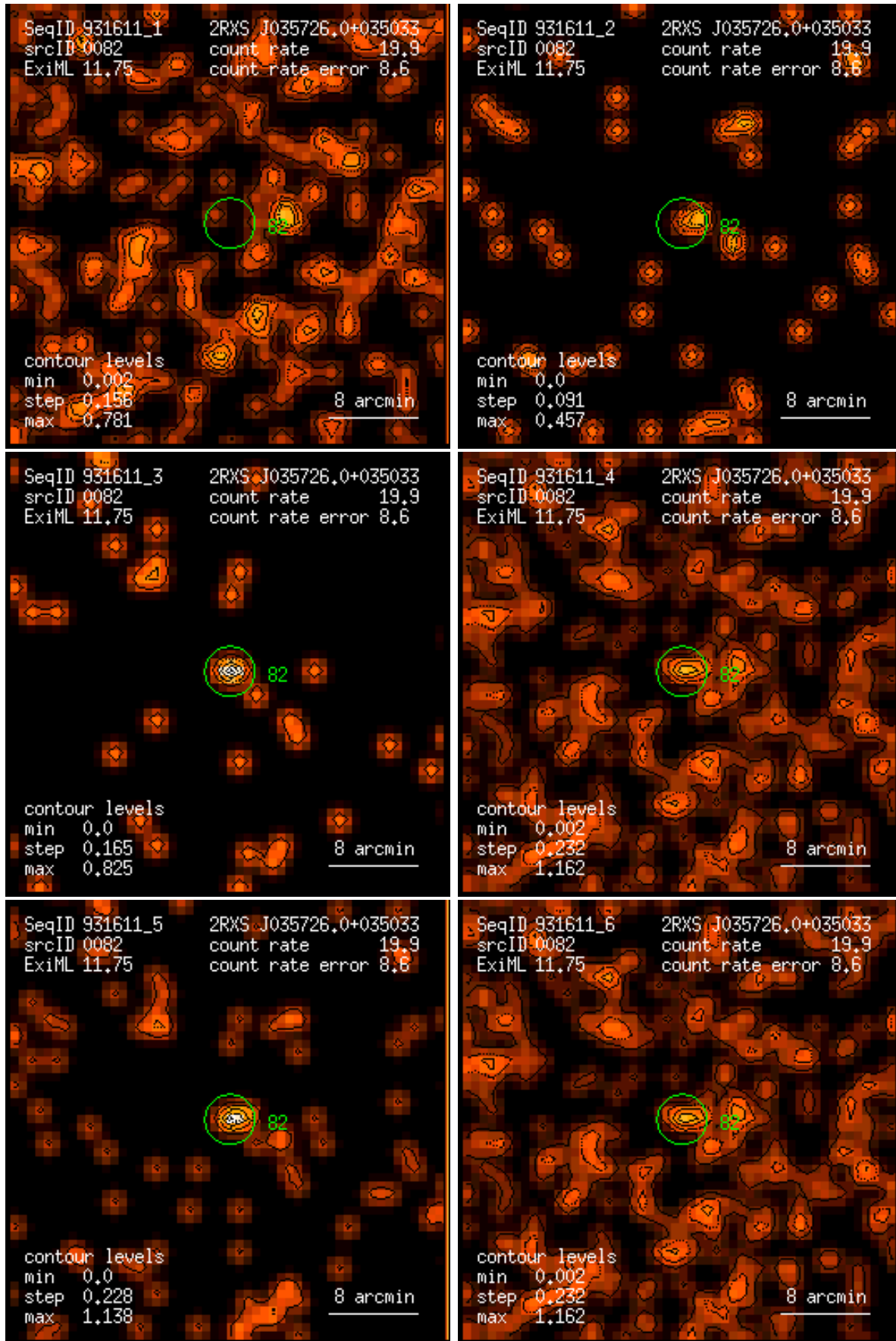
Figure 82: RASS 931611: detection 0082: band rate images, Gaussian filter: (1) PSPC channels 11 – 41, (2) 52 – 90, (3) 91 – 201, (4) 11 – 235, (5) 52 – 201, (6) 11 – 201. Broad band rates in counts/ks. Band rate contour levels in counts/ks/arcmin 2 .
