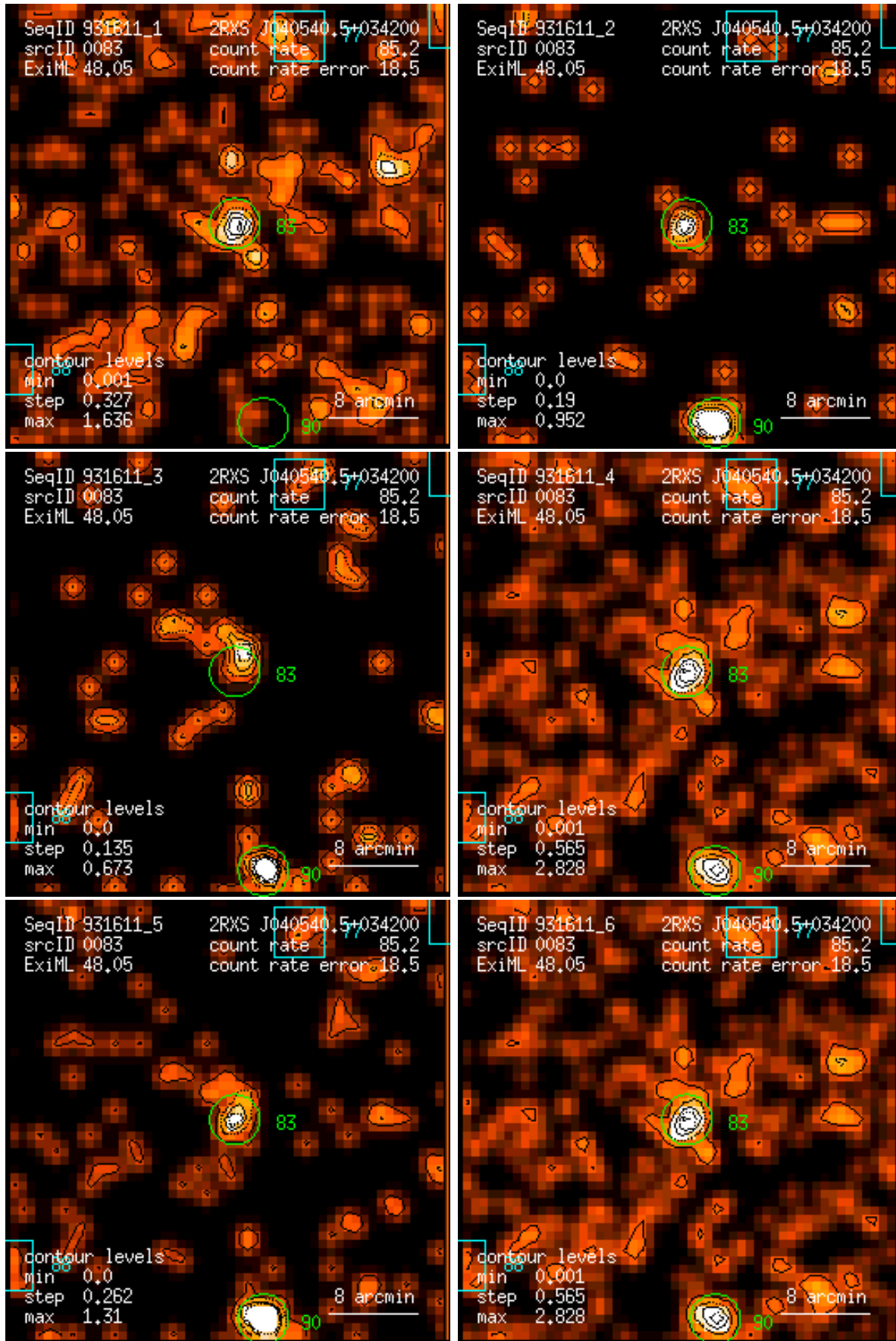
Figure 83: RASS 931611: detection 0083: band rate images, Gaussian filter: (1) PSPC channels 11 – 41, (2) 52 – 90, (3) 91 – 201, (4) 11 – 235, (5) 52 – 201, (6) 11 – 201. Broad band rates in counts/ks. Band rate contour levels in counts/ks/arcmin 2 .
