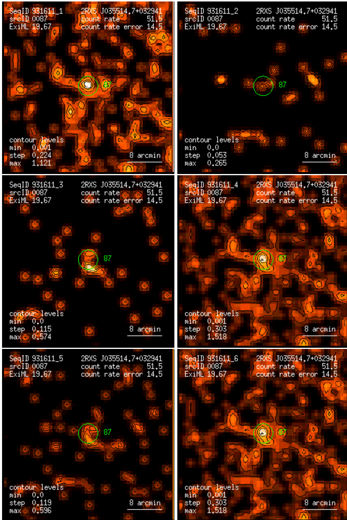
Figure 87: RASS 931611: detection 0087: band rate images, Gaussian filter: (1) PSPC channels 11 – 41, (2) 52 – 90, (3) 91 – 201, (4) 11 – 235, (5) 52 – 201, (6) 11 – 201. Broad band rates in counts/ks. Band rate contour levels in counts/ks/arcmin 2 .
