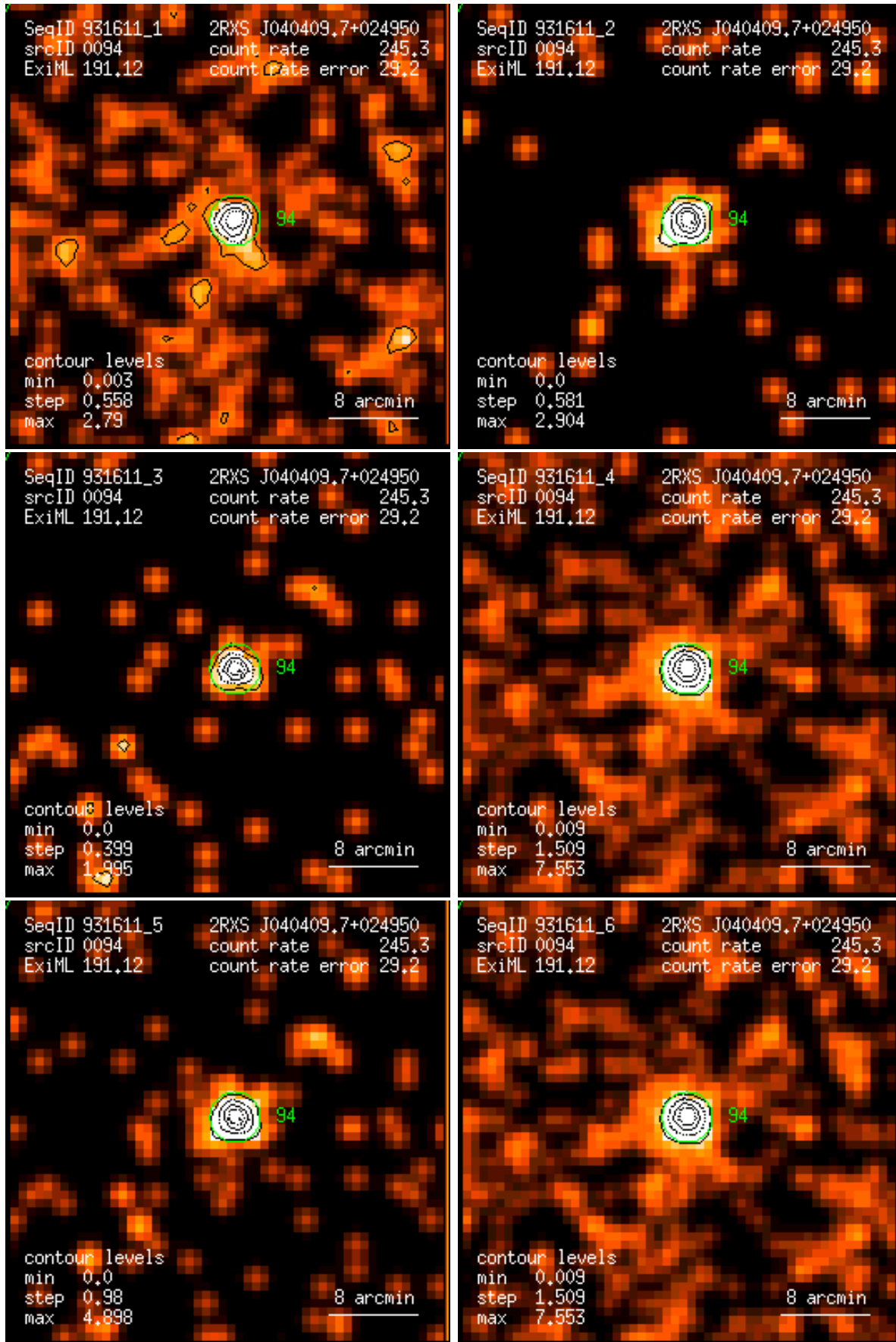
Figure 94: RASS 931611: detection 0094: band rate images, Gaussian filter: (1) PSPC channels 11 – 41, (2) 52 – 90, (3) 91 – 201, (4) 11 – 235, (5) 52 – 201, (6) 11 – 201. Broad band rates in counts/ks. Band rate contour levels in counts/ks/arcmin 2 .
