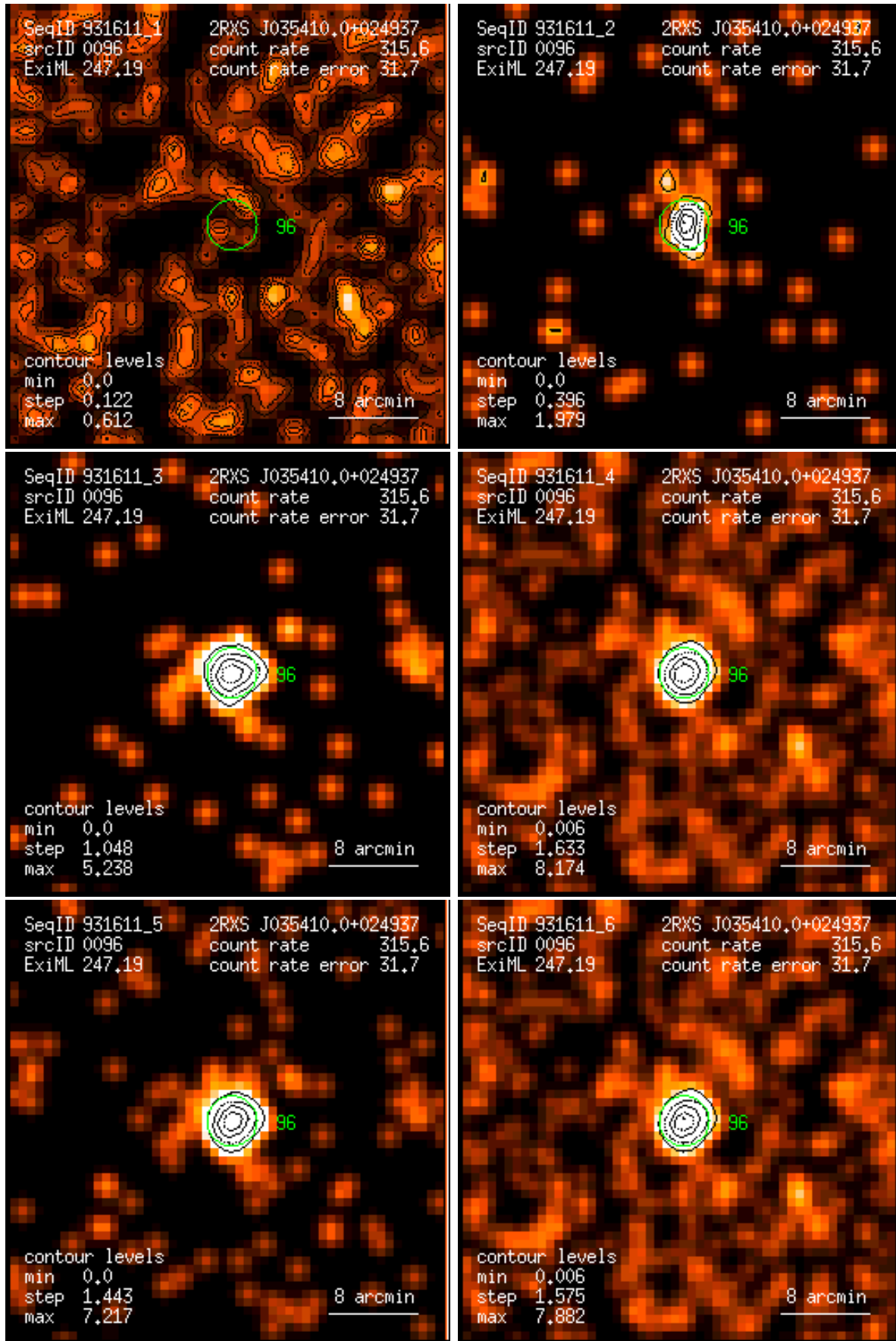
Figure 96: RASS 931611: detection 0096: band rate images, Gaussian filter: (1) PSPC channels 11 – 41, (2) 52 – 90, (3) 91 – 201, (4) 11 – 235, (5) 52 – 201, (6) 11 – 201. Broad band rates in counts/ks. Band rate contour levels in counts/ks/arcmin 2 .
