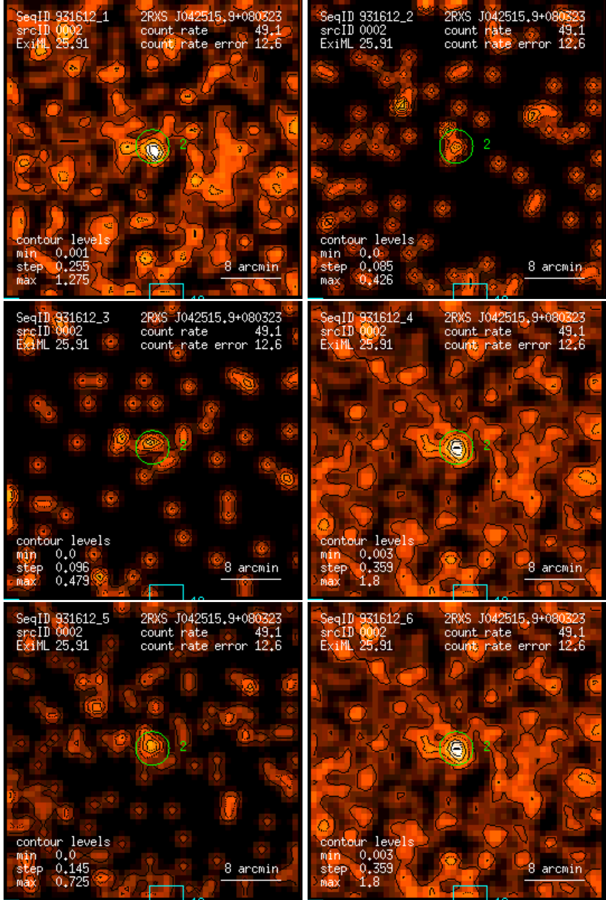
Figure 2: RASS 931612: detection 0002: band rate images, Gaussian filter: (1) PSPC channels 11 – 41, (2) 52 – 90, (3) 91 – 201, (4) 11 – 235, (5) 52 – 201, (6) 11 – 201. Broad band rates in counts/ks. Band rate contour levels in counts/ks/arcmin 2 .
