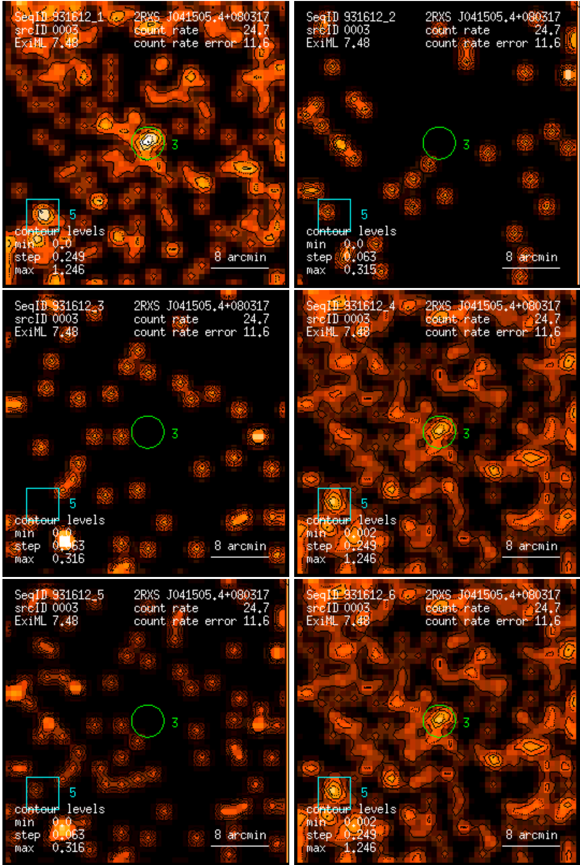
Figure 3: RASS 931612: detection 0003: band rate images, Gaussian filter: (1) PSPC channels 11 – 41, (2) 52 – 90, (3) 91 – 201, (4) 11 – 235, (5) 52 – 201, (6) 11 – 201. Broad band rates in counts/ks. Band rate contour levels in counts/ks/arcmin 2 .
