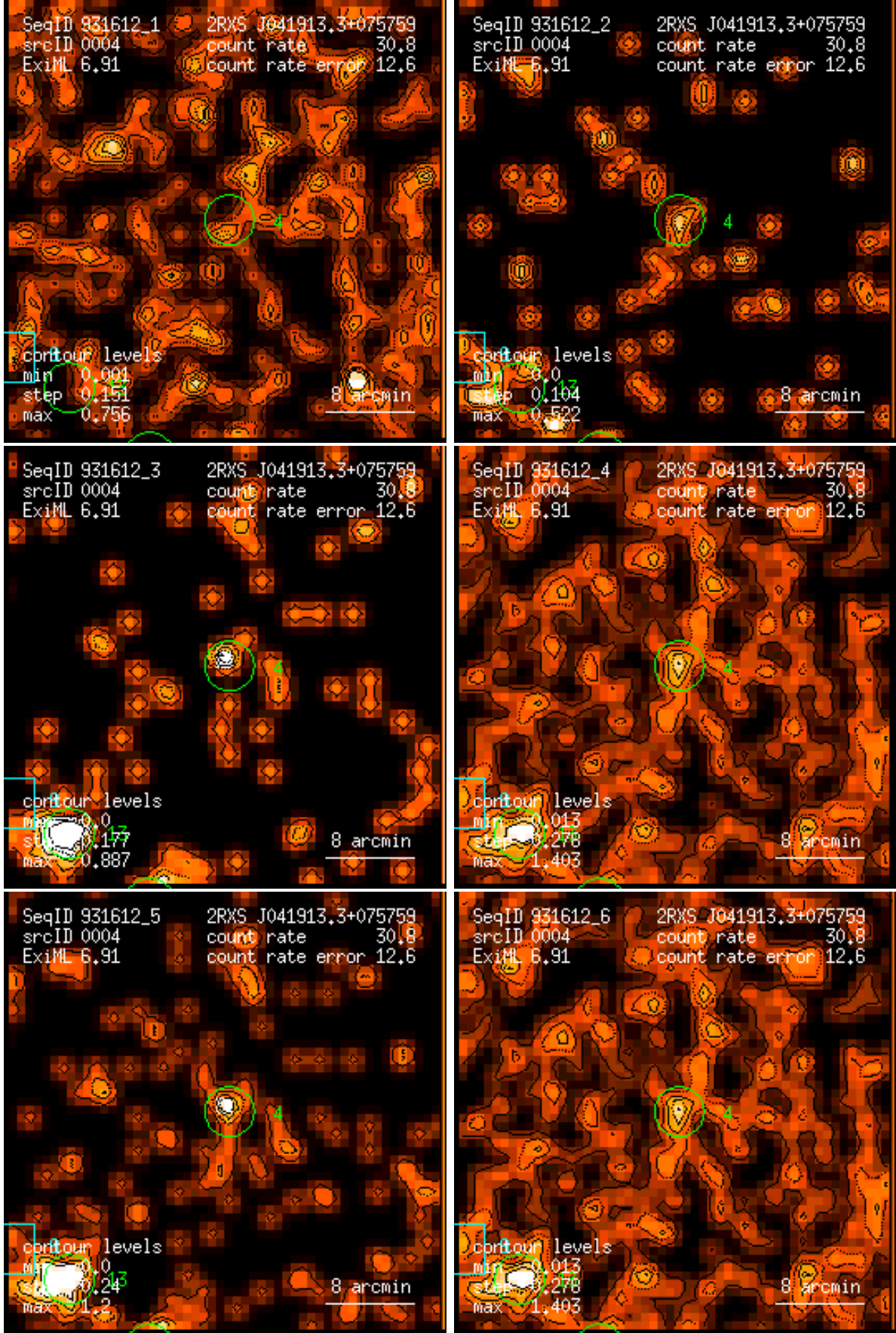
Figure 4: RASS 931612: detection 0004: band rate images, Gaussian filter: (1) PSPC channels 11 – 41, (2) 52 – 90, (3) 91 – 201, (4) 11 – 235, (5) 52 – 201, (6) 11 – 201. Broad band rates in counts/ks. Band rate contour levels in counts/ks/arcmin 2 .
