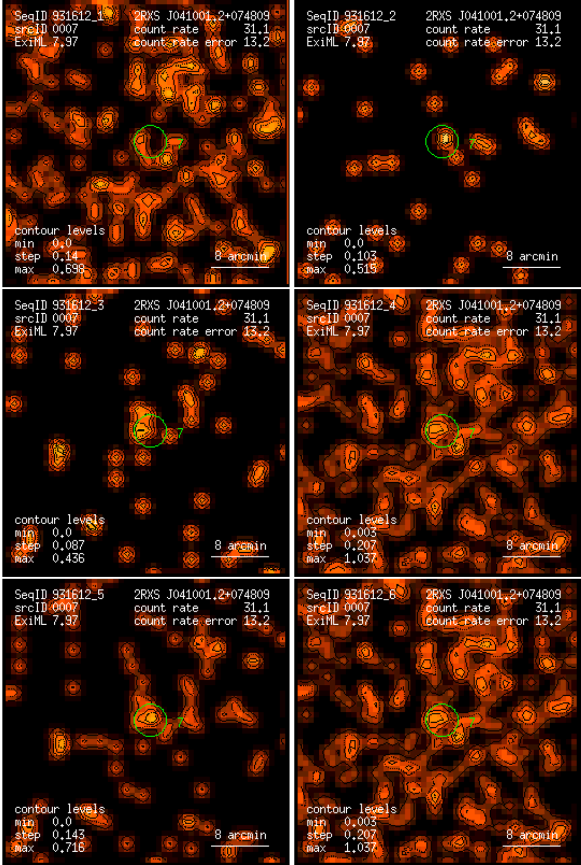
Figure 7: RASS 931612: detection 0007: band rate images, Gaussian filter: (1) PSPC channels 11 – 41, (2) 52 – 90, (3) 91 – 201, (4) 11 – 235, (5) 52 – 201, (6) 11 – 201. Broad band rates in counts/ks. Band rate contour levels in counts/ks/arcmin 2 .
