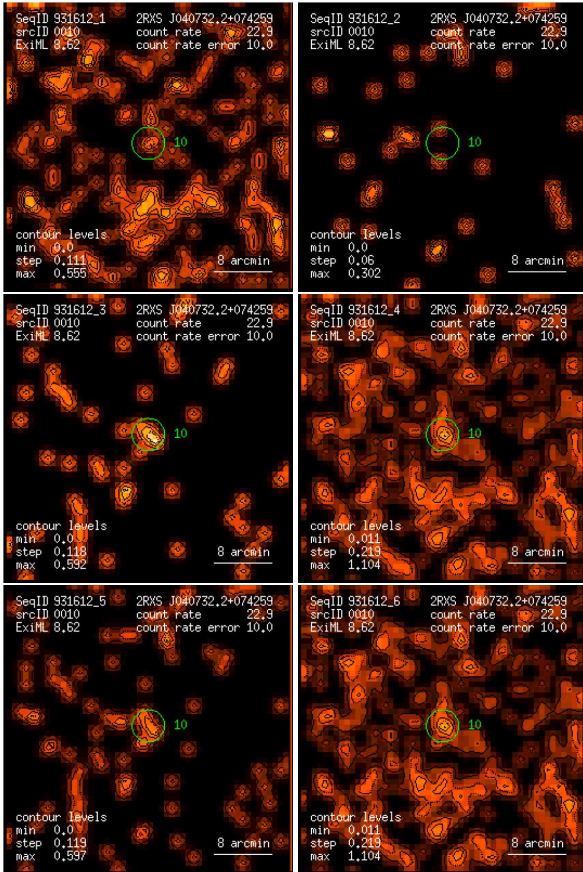
Figure 10: RASS 931612: detection 0010: band rate images, Gaussian filter: (1) PSPC channels 11 – 41, (2) 52 – 90, (3) 91 – 201, (4) 11 – 235, (5) 52 – 201, (6) 11 – 201. Broad band rates in counts/ks. Band rate contour levels in counts/ks/arcmin 2 .
