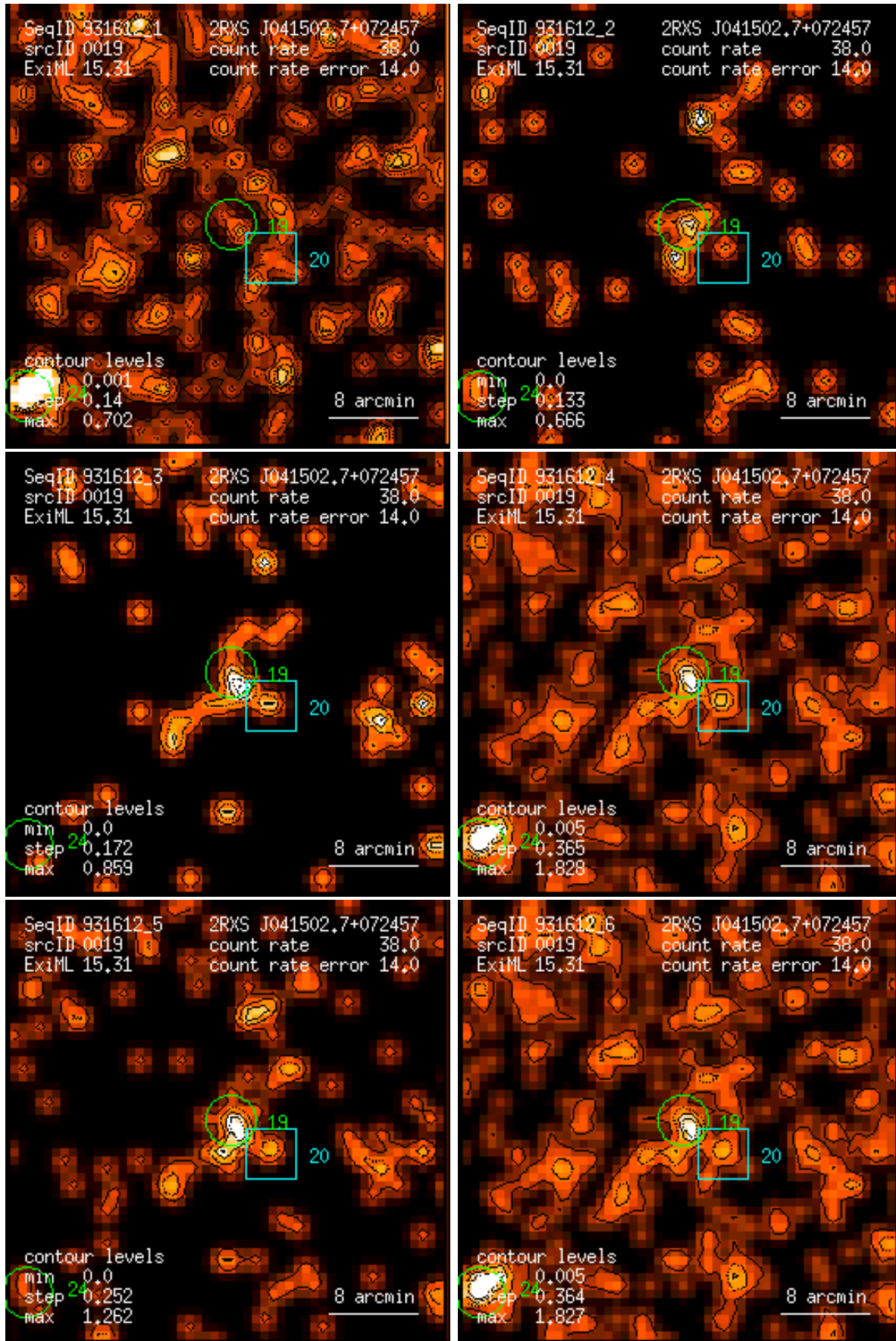
Figure 19: RASS 931612: detection 0019: band rate images, Gaussian filter: (1) PSPC channels 11 – 41, (2) 52 – 90, (3) 91 – 201, (4) 11 – 235, (5) 52 – 201, (6) 11 – 201. Broad band rates in counts/ks. Band rate contour levels in counts/ks/arcmin 2 .
