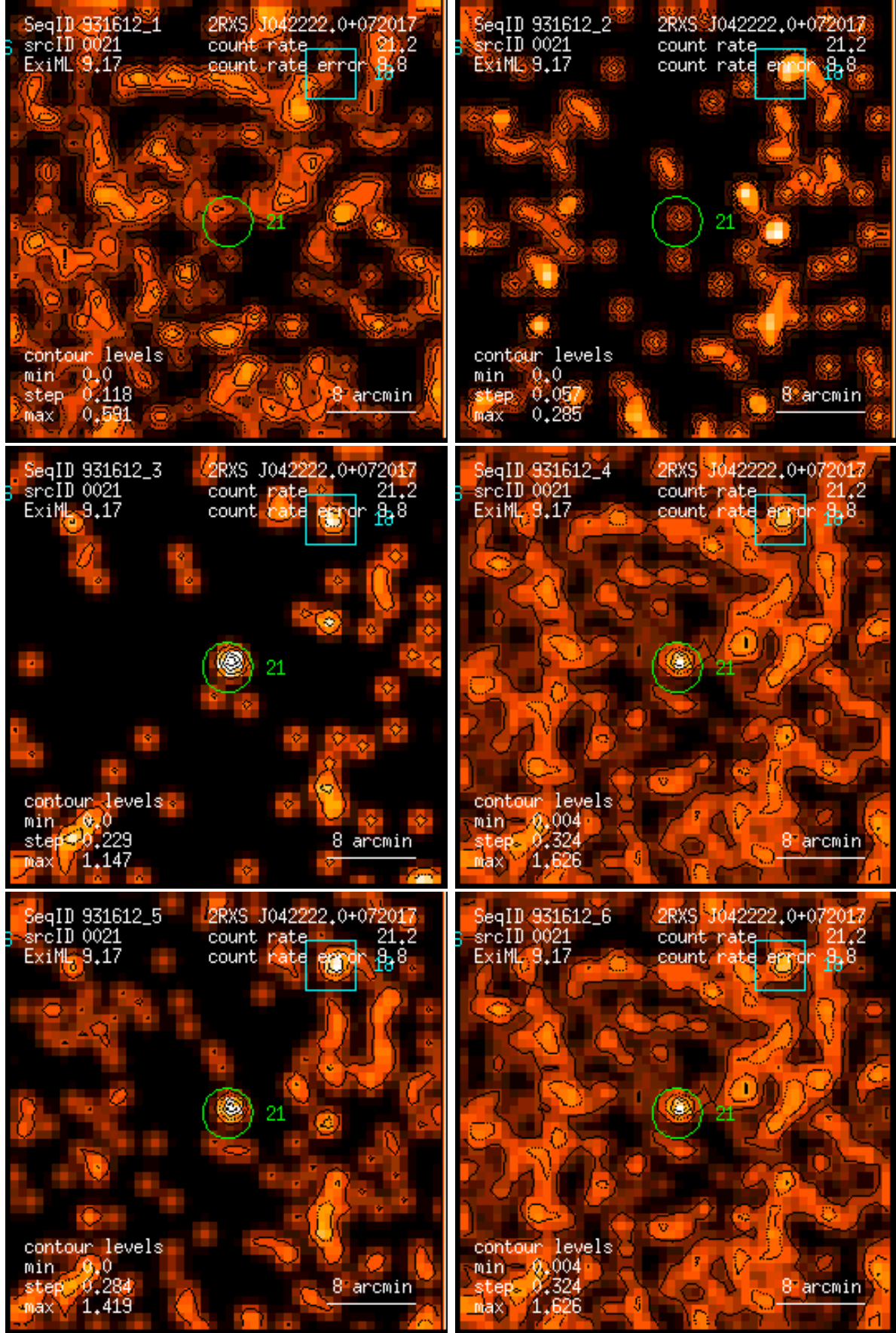
Figure 21: RASS 931612: detection 0021: band rate images, Gaussian filter: (1) PSPC channels 11 – 41, (2) 52 – 90, (3) 91 – 201, (4) 11 – 235, (5) 52 – 201, (6) 11 – 201. Broad band rates in counts/ks. Band rate contour levels in counts/ks/arcmin 2 .
