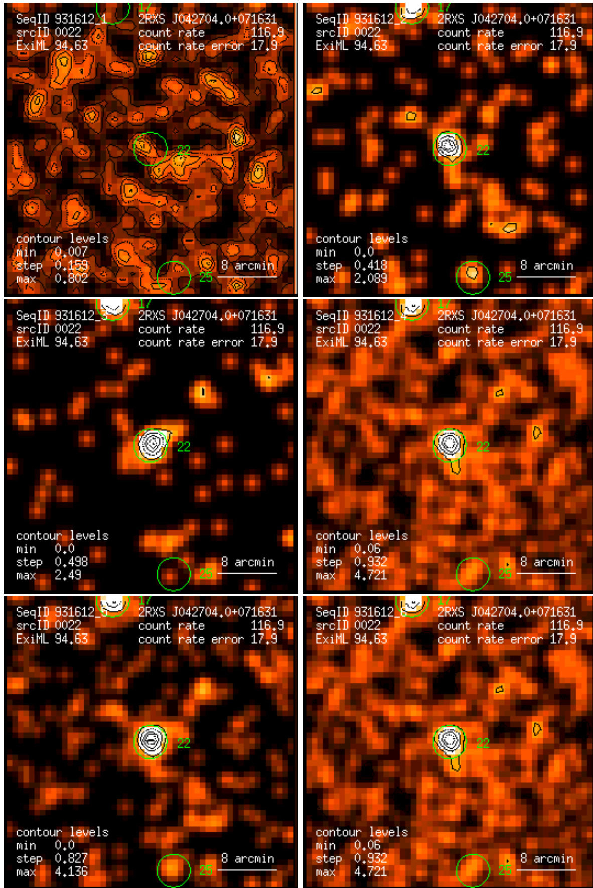
Figure 22: RASS 931612: detection 0022: band rate images, Gaussian filter: (1) PSPC channels 11 – 41, (2) 52 – 90, (3) 91 – 201, (4) 11 – 235, (5) 52 – 201, (6) 11 – 201. Broad band rates in counts/ks. Band rate contour levels in counts/ks/arcmin 2 .
