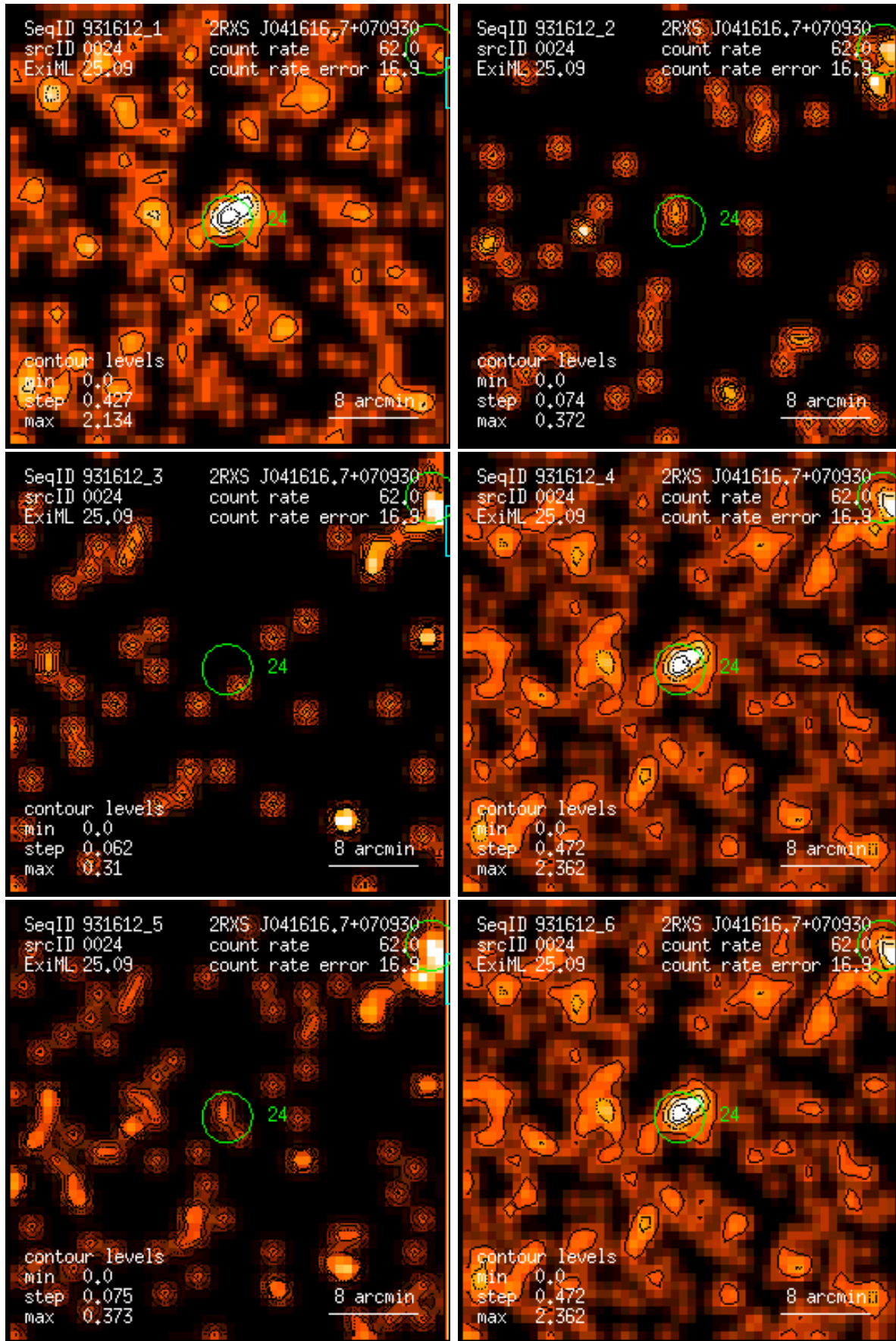
Figure 24: RASS 931612: detection 0024: band rate images, Gaussian filter: (1) PSPC channels 11 – 41, (2) 52 – 90, (3) 91 – 201, (4) 11 – 235, (5) 52 – 201, (6) 11 – 201. Broad band rates in counts/ks. Band rate contour levels in counts/ks/arcmin 2 .
