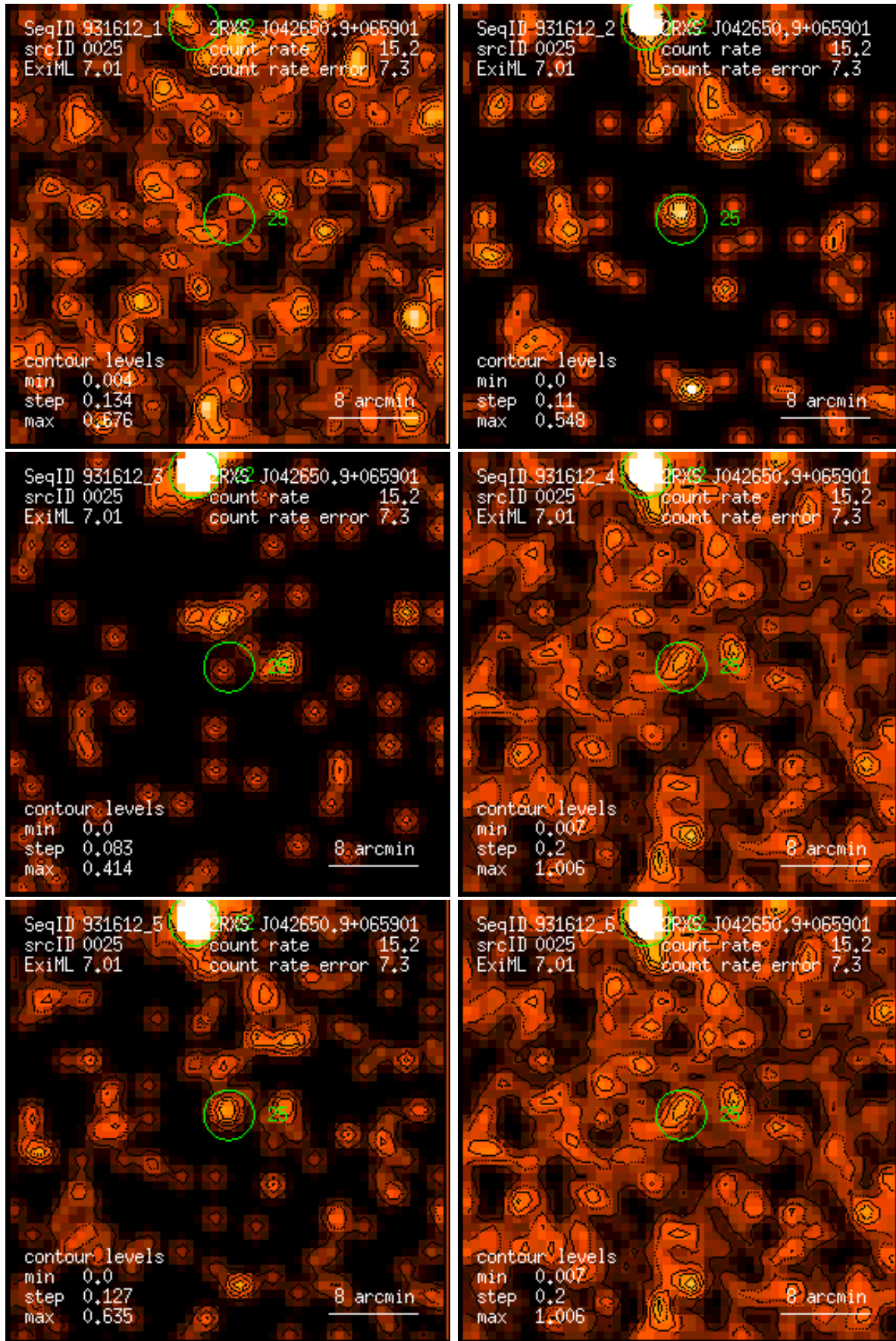
Figure 25: RASS 931612: detection 0025: band rate images, Gaussian filter: (1) PSPC channels 11 – 41, (2) 52 – 90, (3) 91 – 201, (4) 11 – 235, (5) 52 – 201, (6) 11 – 201. Broad band rates in counts/ks. Band rate contour levels in counts/ks/arcmin 2 .
