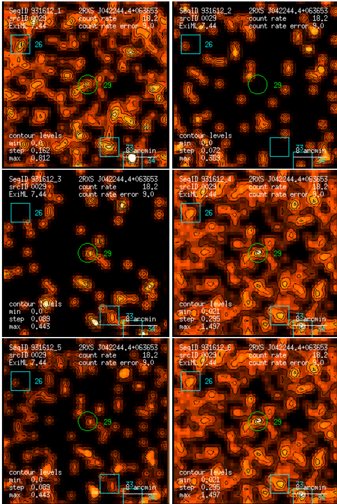
Figure 29: RASS 931612: detection 0029: band rate images, Gaussian filter: (1) PSPC channels 11 – 41, (2) 52 – 90, (3) 91 – 201, (4) 11 – 235, (5) 52 – 201, (6) 11 – 201. Broad band rates in counts/ks. Band rate contour levels in counts/ks/arcmin 2 .
