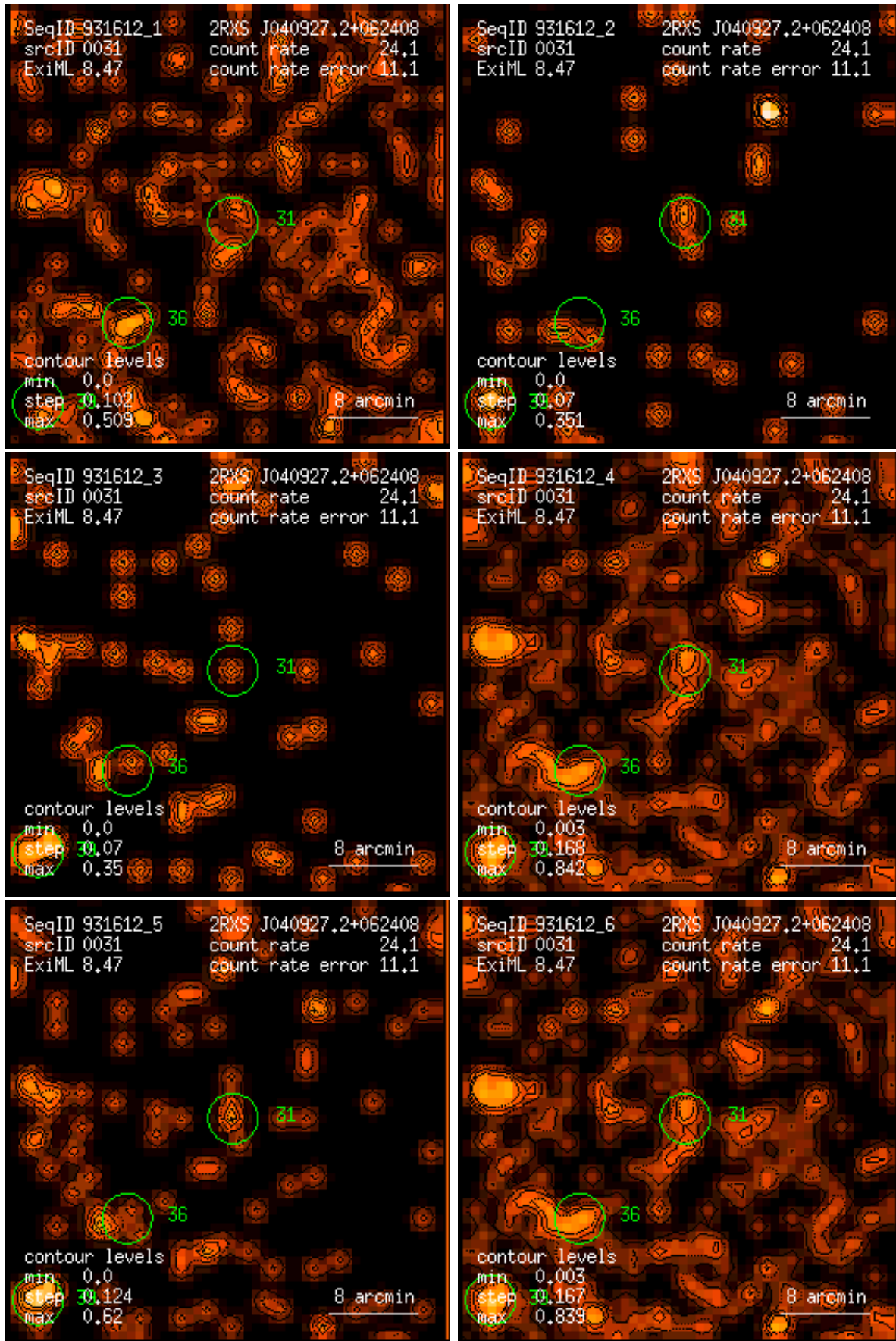
Figure 31: RASS 931612: detection 0031: band rate images, Gaussian filter: (1) PSPC channels 11 – 41, (2) 52 – 90, (3) 91 – 201, (4) 11 – 235, (5) 52 – 201, (6) 11 – 201. Broad band rates in counts/ks. Band rate contour levels in counts/ks/arcmin 2 .
