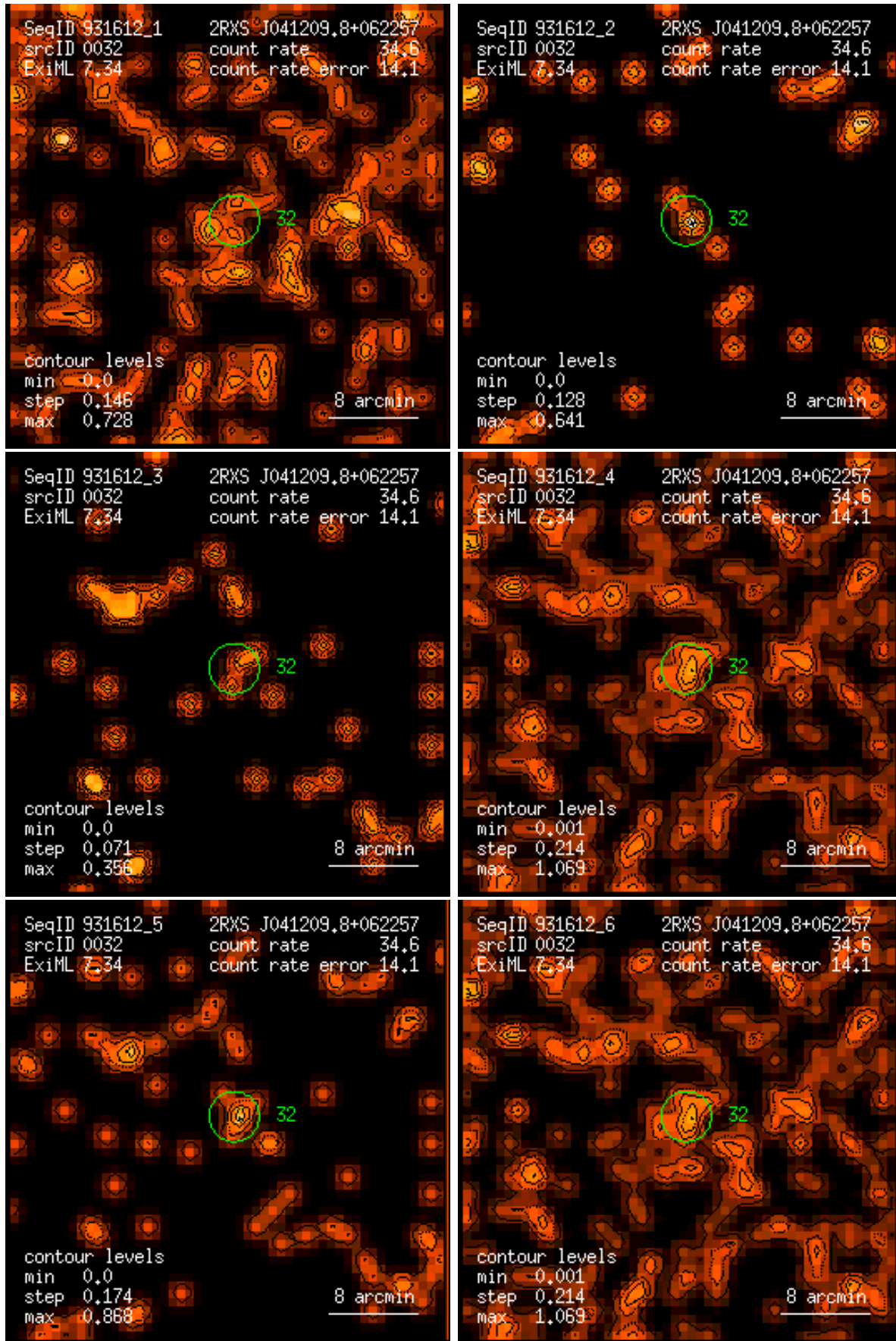
Figure 32: RASS 931612: detection 0032: band rate images, Gaussian filter: (1) PSPC channels 11 – 41, (2) 52 – 90, (3) 91 – 201, (4) 11 – 235, (5) 52 – 201, (6) 11 – 201. Broad band rates in counts/ks. Band rate contour levels in counts/ks/arcmin 2 .
