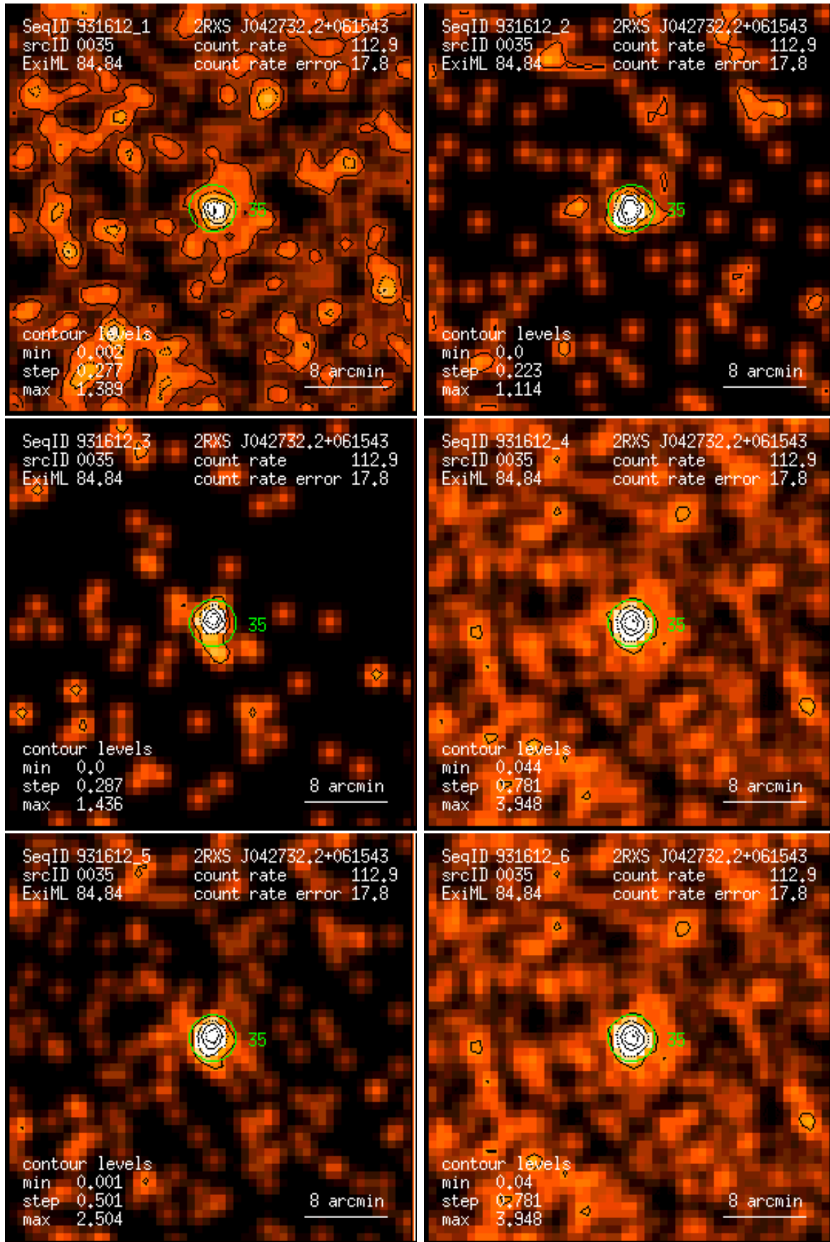
Figure 35: RASS 931612: detection 0035: band rate images, Gaussian filter: (1) PSPC channels 11 – 41, (2) 52 – 90, (3) 91 – 201, (4) 11 – 235, (5) 52 – 201, (6) 11 – 201. Broad band rates in counts/ks. Band rate contour levels in counts/ks/arcmin 2 .
