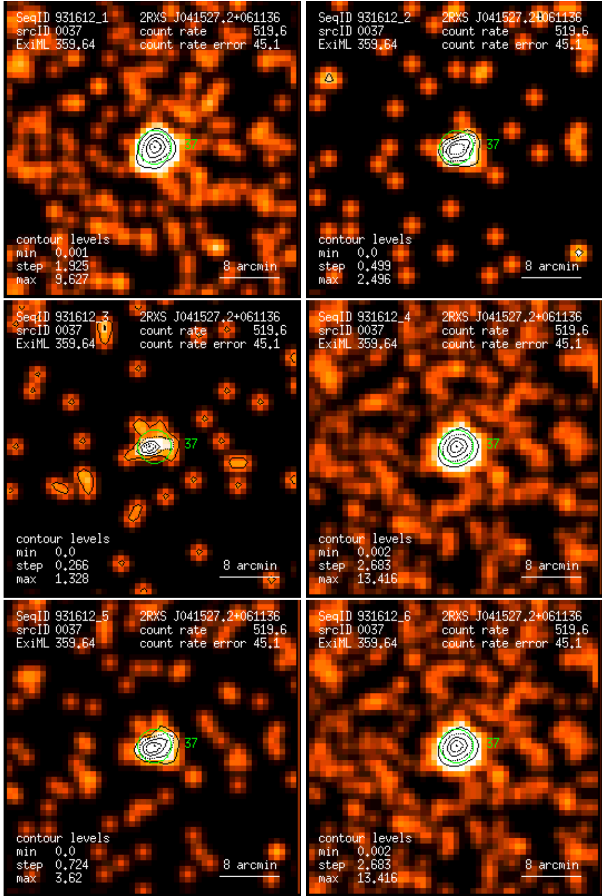
Figure 37: RASS 931612: detection 0037: band rate images, Gaussian filter: (1) PSPC channels 11 – 41, (2) 52 – 90, (3) 91 – 201, (4) 11 – 235, (5) 52 – 201, (6) 11 – 201. Broad band rates in counts/ks. Band rate contour levels in counts/ks/arcmin 2 .
