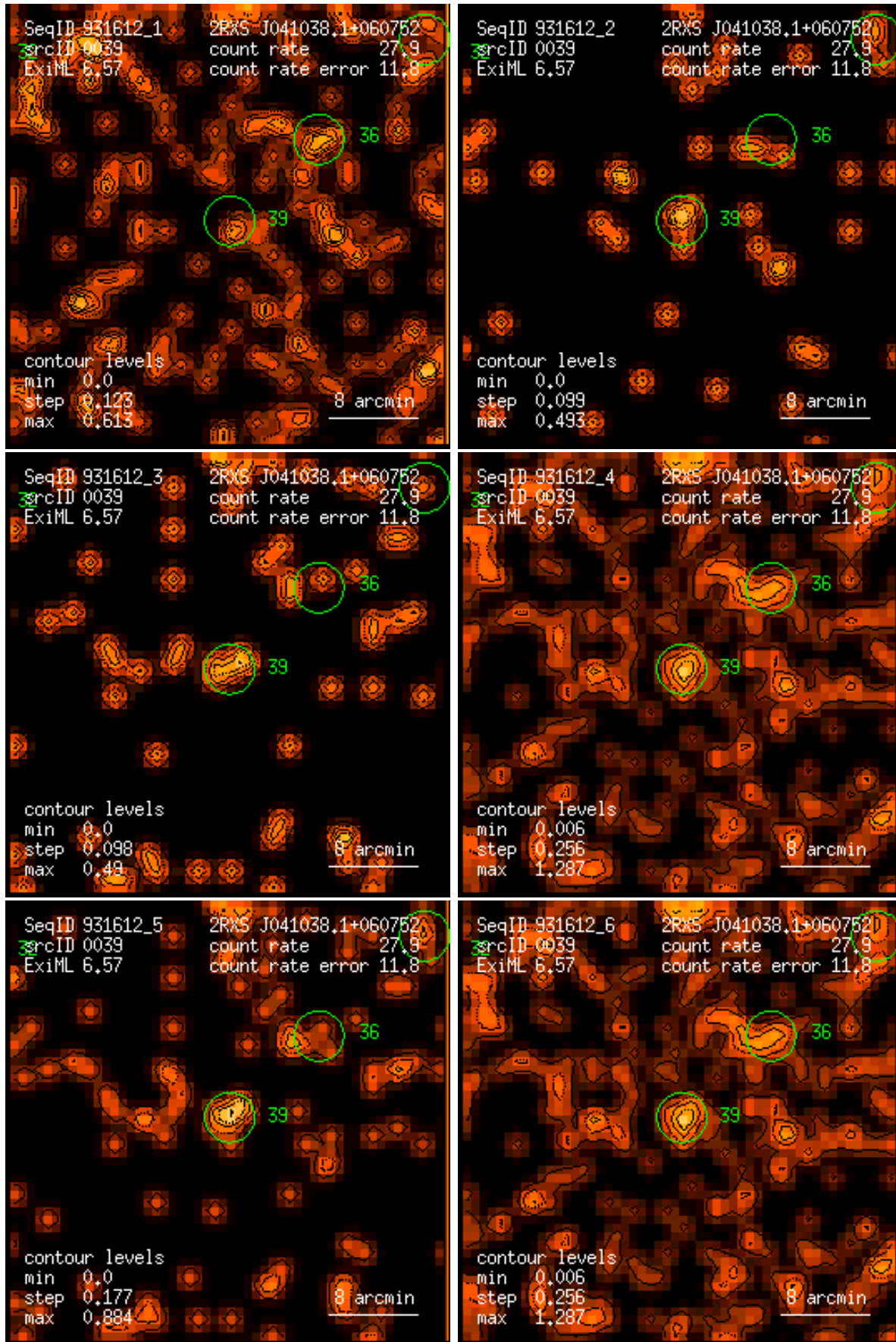
Figure 39: RASS 931612: detection 0039: band rate images, Gaussian filter: (1) PSPC channels 11 – 41, (2) 52 – 90, (3) 91 – 201, (4) 11 – 235, (5) 52 – 201, (6) 11 – 201. Broad band rates in counts/ks. Band rate contour levels in counts/ks/arcmin 2 .
