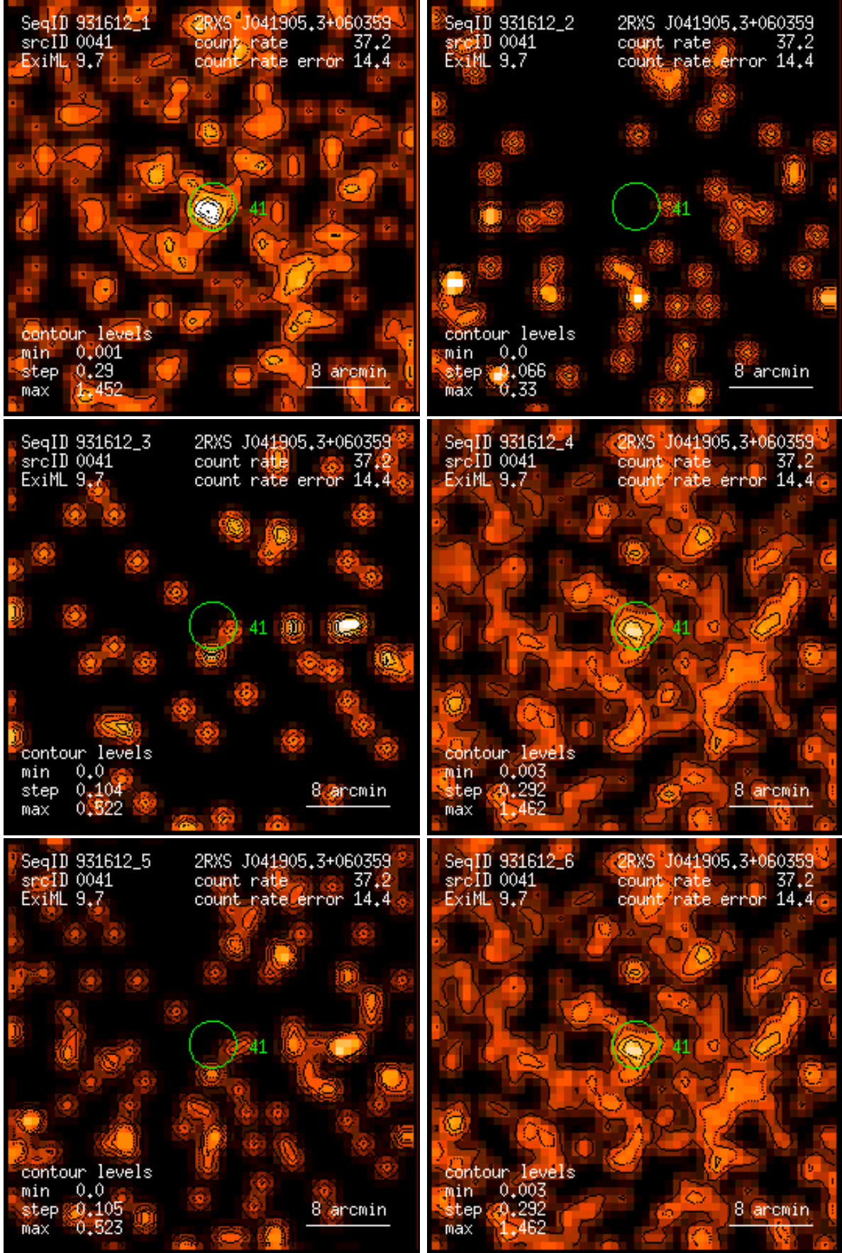
Figure 41: RASS 931612: detection 0041: band rate images, Gaussian filter: (1) PSPC channels 11 – 41, (2) 52 – 90, (3) 91 – 201, (4) 11 – 235, (5) 52 – 201, (6) 11 – 201. Broad band rates in counts/ks. Band rate contour levels in counts/ks/arcmin 2 .
