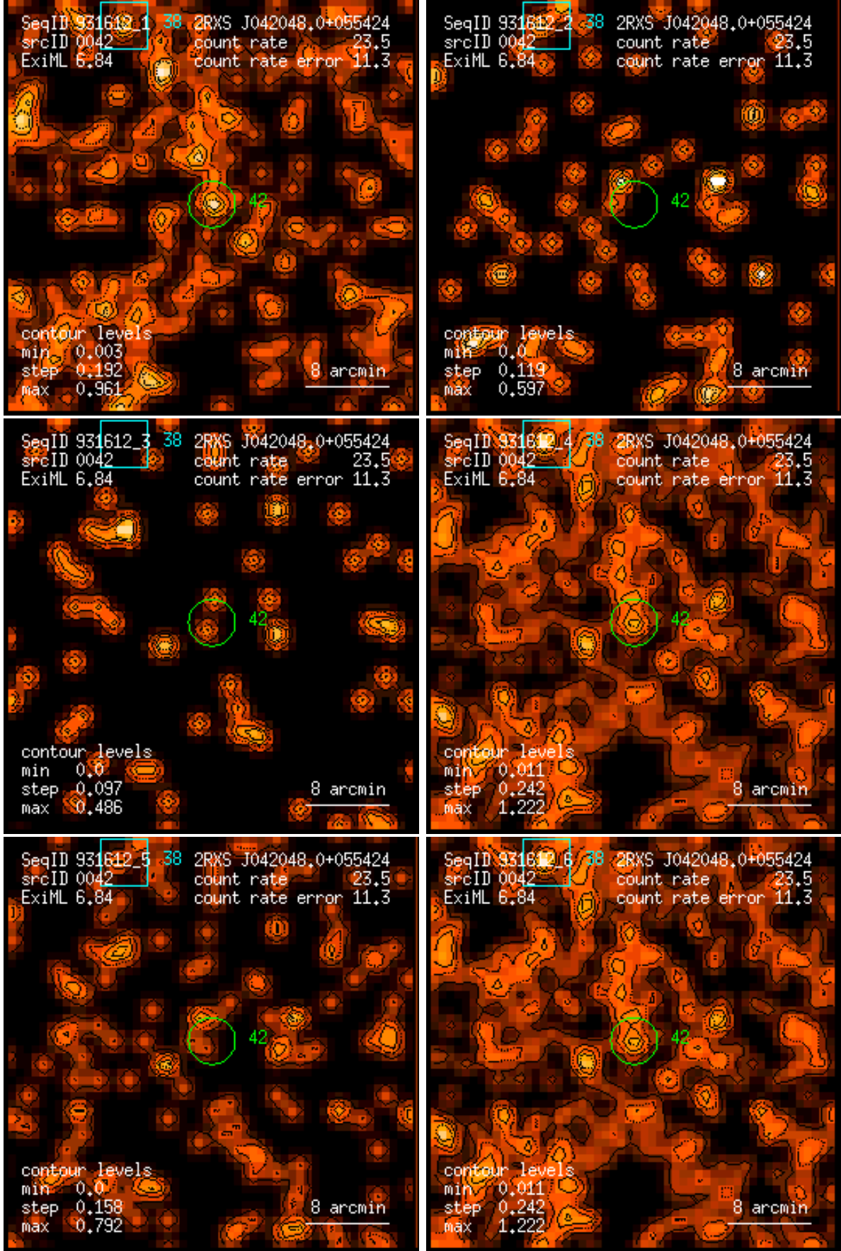
Figure 42: RASS 931612: detection 0042: band rate images, Gaussian filter: (1) PSPC channels 11 – 41, (2) 52 – 90, (3) 91 – 201, (4) 11 – 235, (5) 52 – 201, (6) 11 – 201. Broad band rates in counts/ks. Band rate contour levels in counts/ks/arcmin 2 .
