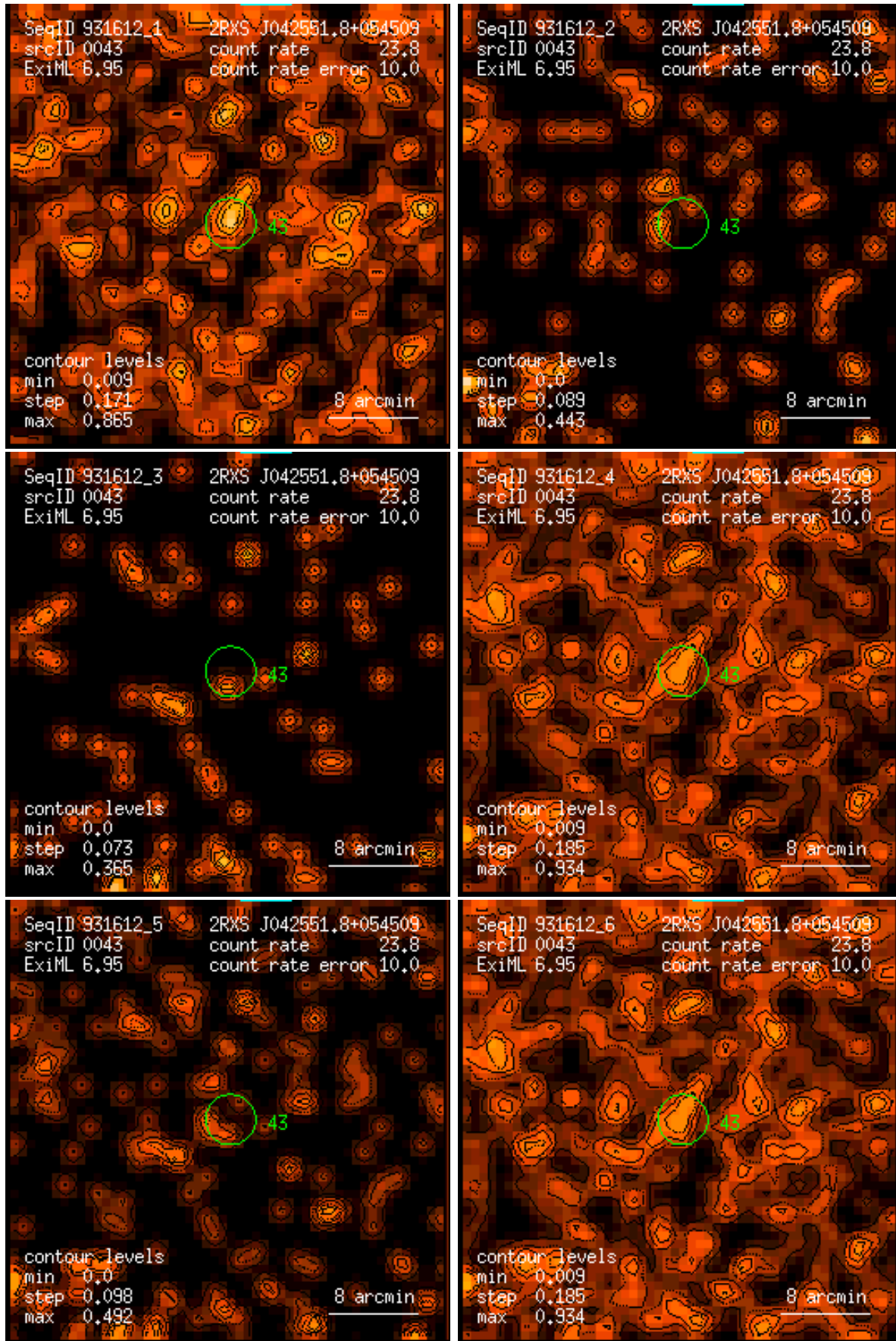
Figure 43: RASS 931612: detection 0043: band rate images, Gaussian filter: (1) PSPC channels 11 – 41, (2) 52 – 90, (3) 91 – 201, (4) 11 – 235, (5) 52 – 201, (6) 11 – 201. Broad band rates in counts/ks. Band rate contour levels in counts/ks/arcmin 2 .
