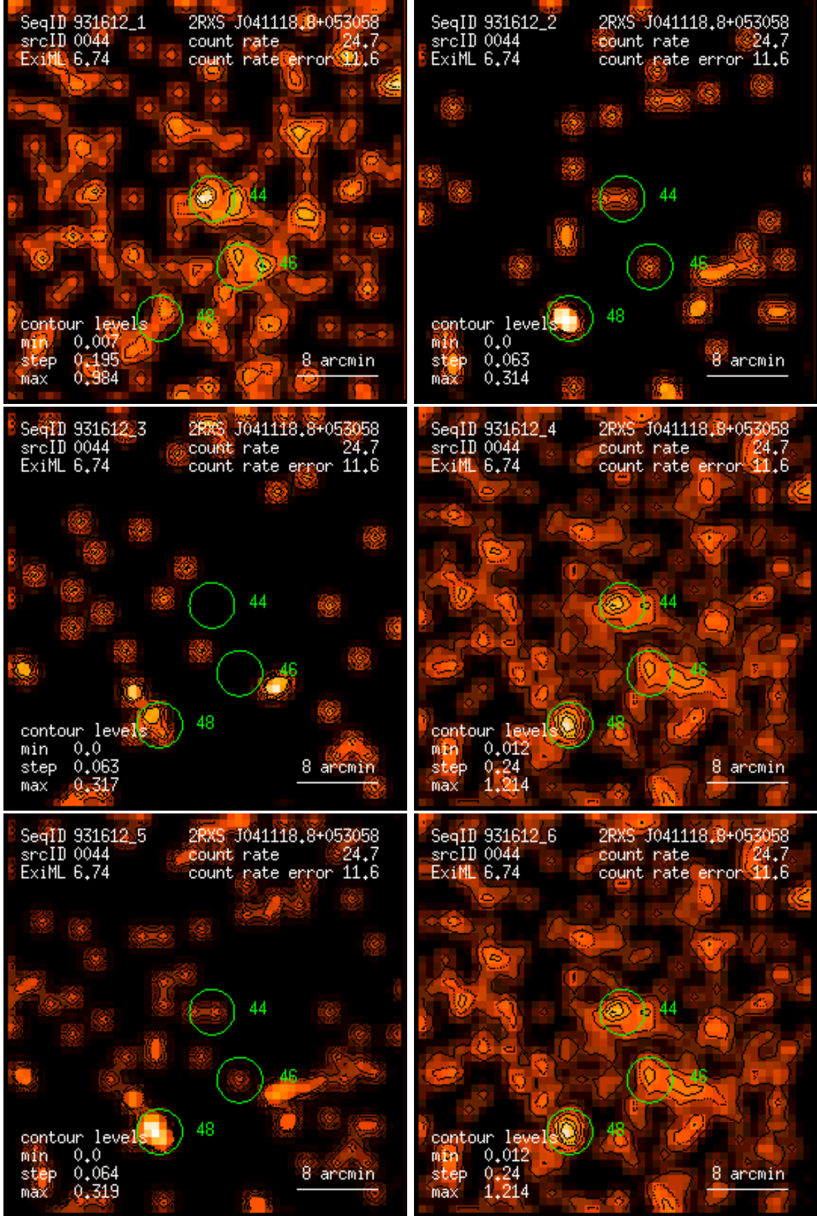
Figure 44: RASS 931612: detection 0044: band rate images, Gaussian filter: (1) PSPC channels 11 – 41, (2) 52 – 90, (3) 91 – 201, (4) 11 – 235, (5) 52 – 201, (6) 11 – 201. Broad band rates in counts/ks. Band rate contour levels in counts/ks/arcmin 2 .
