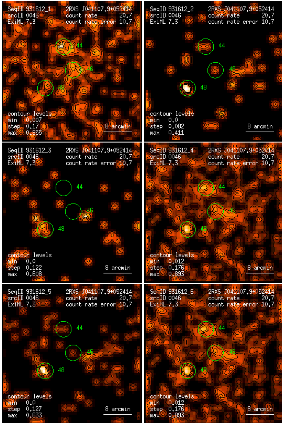
Figure 46: RASS 931612: detection 0046: band rate images, Gaussian filter: (1) PSPC channels 11 – 41, (2) 52 – 90, (3) 91 – 201, (4) 11 – 235, (5) 52 – 201, (6) 11 – 201. Broad band rates in counts/ks. Band rate contour levels in counts/ks/arcmin 2 .
