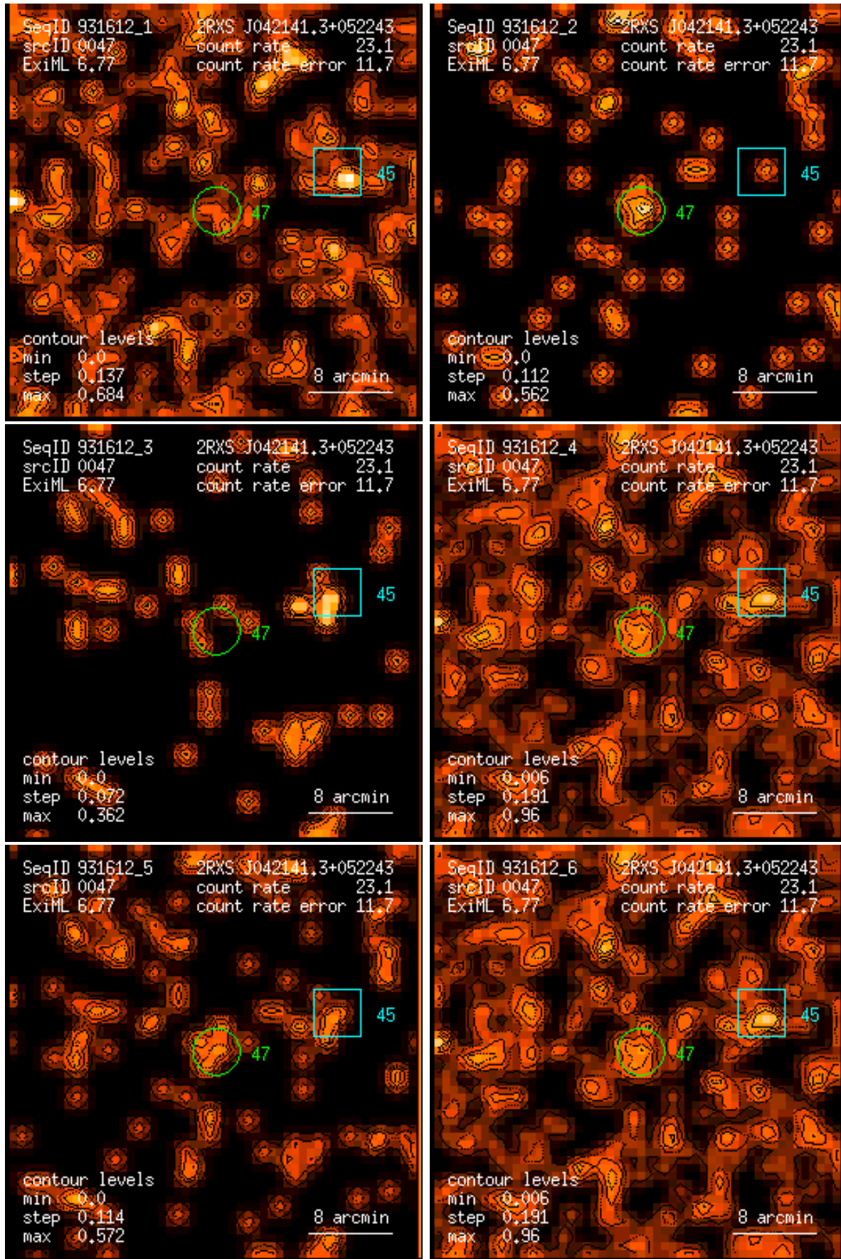
Figure 47: RASS 931612: detection 0047: band rate images, Gaussian filter: (1) PSPC channels 11 – 41, (2) 52 – 90, (3) 91 – 201, (4) 11 – 235, (5) 52 – 201, (6) 11 – 201. Broad band rates in counts/ks. Band rate contour levels in counts/ks/arcmin 2 .
