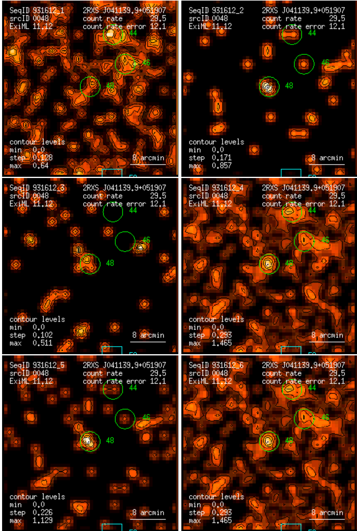
Figure 48: RASS 931612: detection 0048: band rate images, Gaussian filter: (1) PSPC channels 11 – 41, (2) 52 – 90, (3) 91 – 201, (4) 11 – 235, (5) 52 – 201, (6) 11 – 201. Broad band rates in counts/ks. Band rate contour levels in counts/ks/arcmin 2 .
