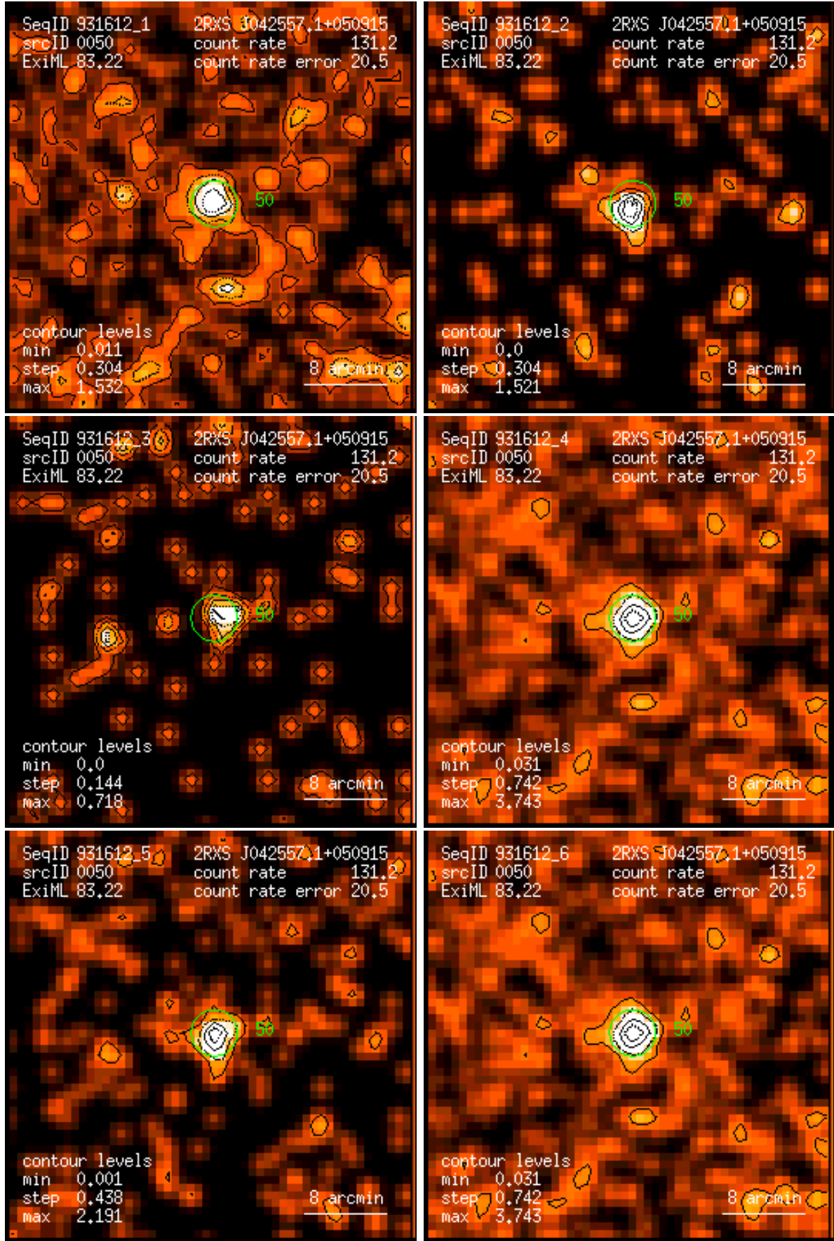
Figure 50: RASS 931612: detection 0050: band rate images, Gaussian filter: (1) PSPC channels 11 – 41, (2) 52 – 90, (3) 91 – 201, (4) 11 – 235, (5) 52 – 201, (6) 11 – 201. Broad band rates in counts/ks. Band rate contour levels in counts/ks/arcmin 2 .
