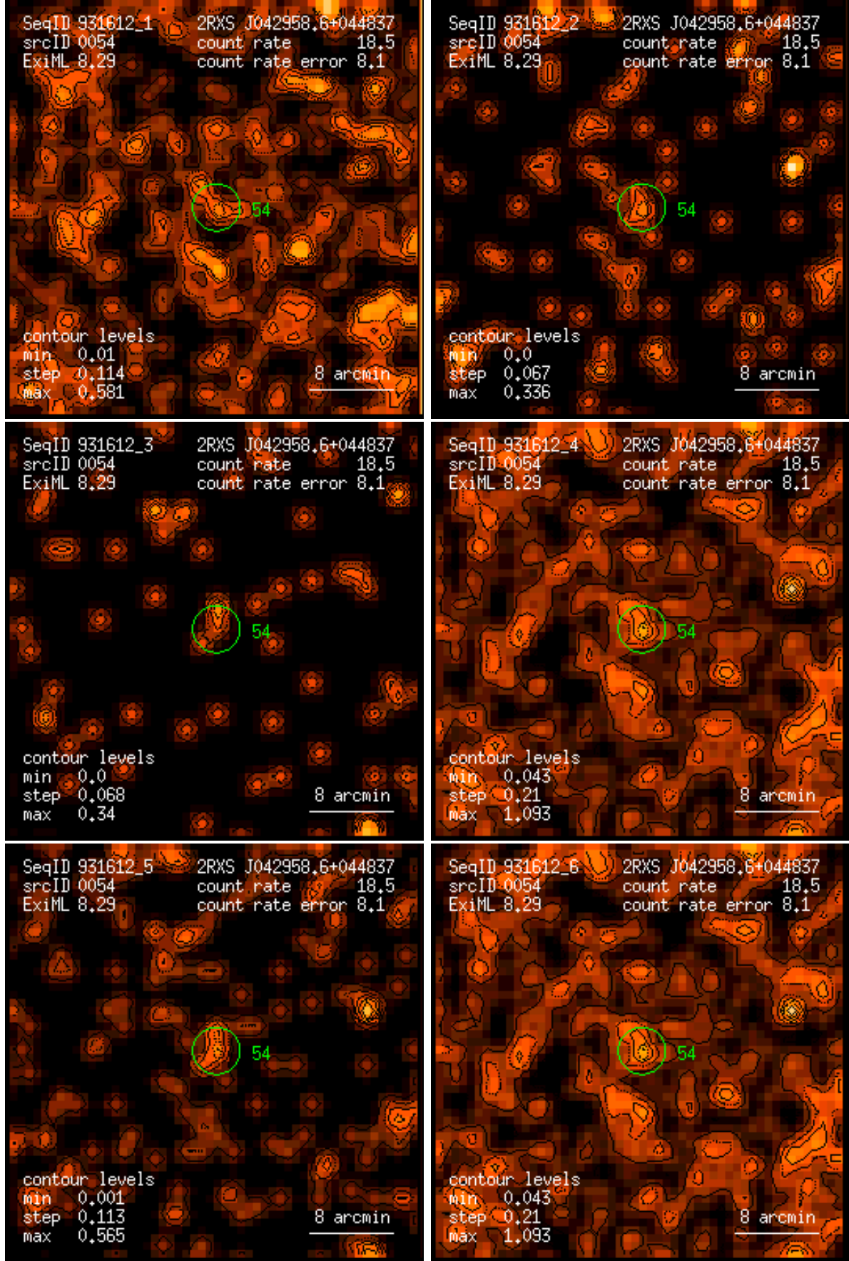
Figure 54: RASS 931612: detection 0054: band rate images, Gaussian filter: (1) PSPC channels 11 – 41, (2) 52 – 90, (3) 91 – 201, (4) 11 – 235, (5) 52 – 201, (6) 11 – 201. Broad band rates in counts/ks. Band rate contour levels in counts/ks/arcmin 2 .
