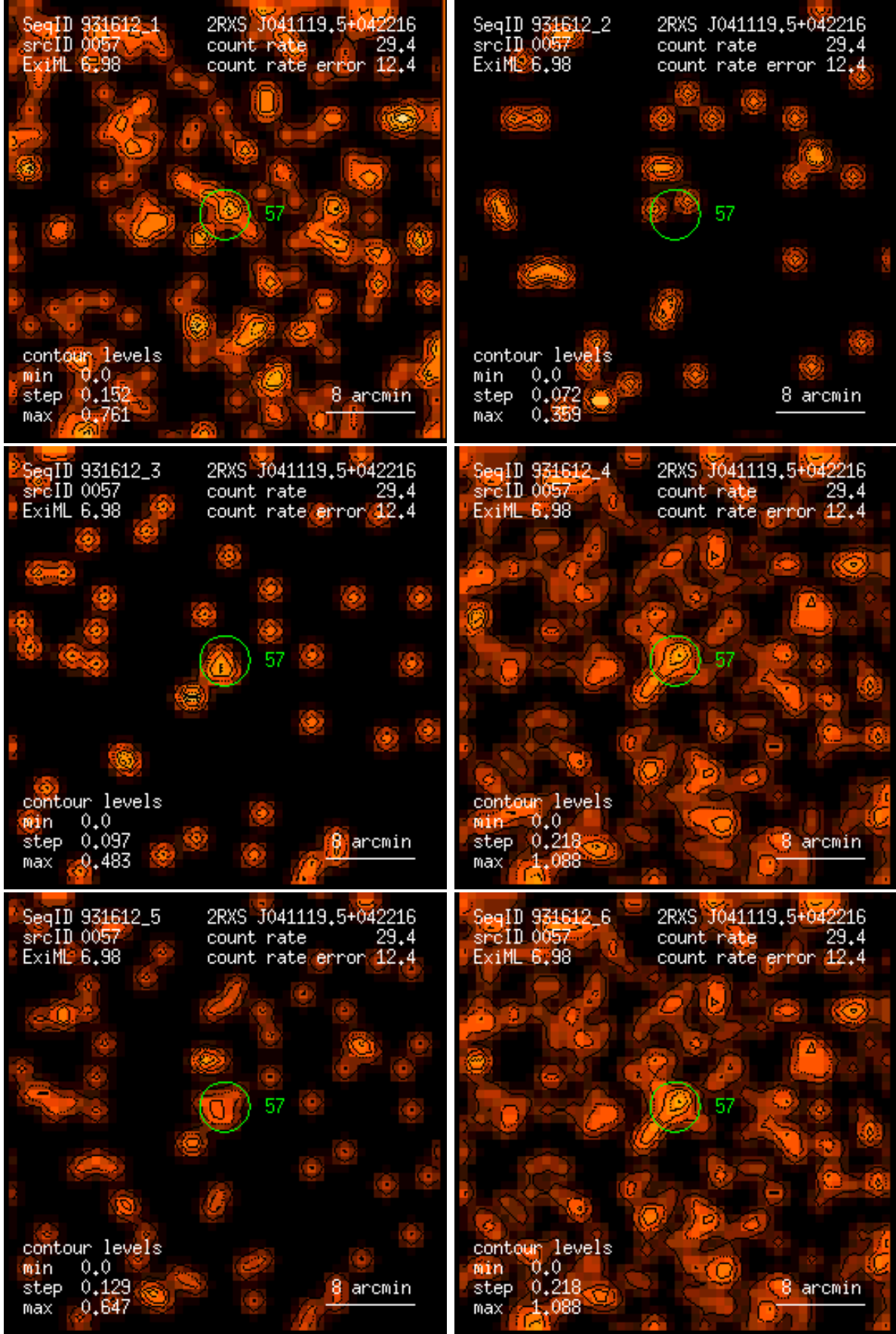
Figure 57: RASS 931612: detection 0057: band rate images, Gaussian filter: (1) PSPC channels 11 – 41, (2) 52 – 90, (3) 91 – 201, (4) 11 – 235, (5) 52 – 201, (6) 11 – 201. Broad band rates in counts/ks. Band rate contour levels in counts/ks/arcmin 2 .
