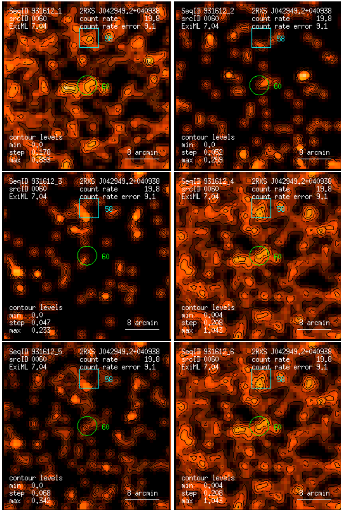
Figure 60: RASS 931612: detection 0060: band rate images, Gaussian filter: (1) PSPC channels 11 – 41, (2) 52 – 90, (3) 91 – 201, (4) 11 – 235, (5) 52 – 201, (6) 11 – 201. Broad band rates in counts/ks. Band rate contour levels in counts/ks/arcmin 2 .
