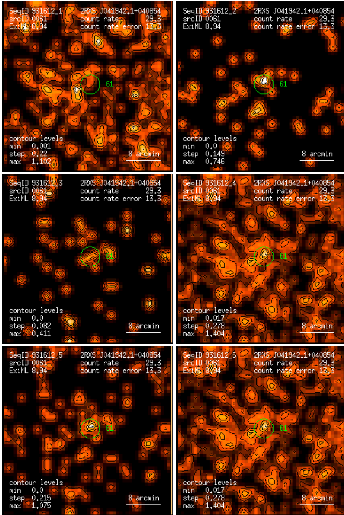
Figure 61: RASS 931612: detection 0061: band rate images, Gaussian filter: (1) PSPC channels 11 – 41, (2) 52 – 90, (3) 91 – 201, (4) 11 – 235, (5) 52 – 201, (6) 11 – 201. Broad band rates in counts/ks. Band rate contour levels in counts/ks/arcmin 2 .
