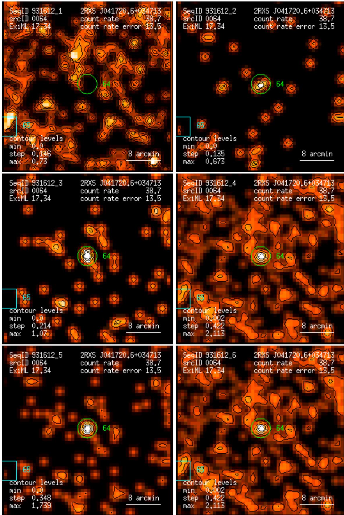
Figure 64: RASS 931612: detection 0064: band rate images, Gaussian filter: (1) PSPC channels 11 – 41, (2) 52 – 90, (3) 91 – 201, (4) 11 – 235, (5) 52 – 201, (6) 11 – 201. Broad band rates in counts/ks. Band rate contour levels in counts/ks/arcmin 2 .
