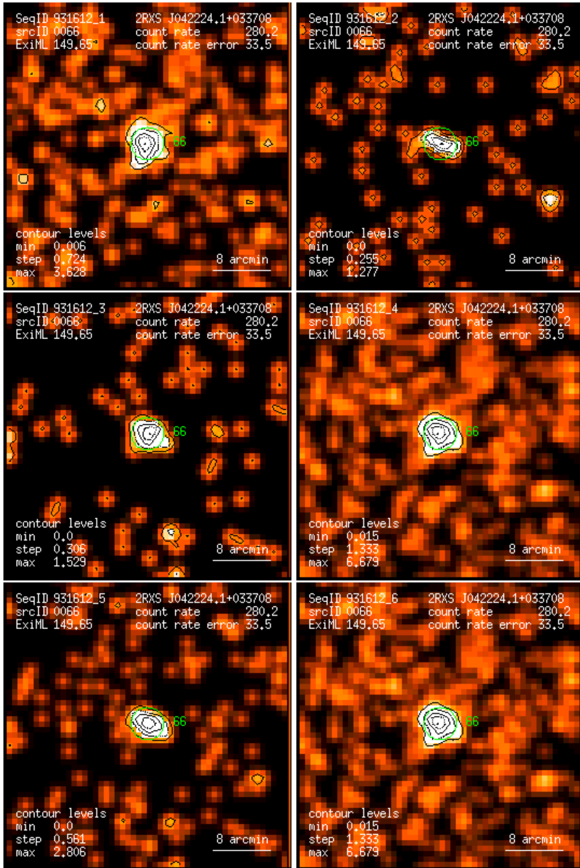
Figure 66: RASS 931612: detection 0066: band rate images, Gaussian filter: (1) PSPC channels 11 – 41, (2) 52 – 90, (3) 91 – 201, (4) 11 – 235, (5) 52 – 201, (6) 11 – 201. Broad band rates in counts/ks. Band rate contour levels in counts/ks/arcmin 2 .
