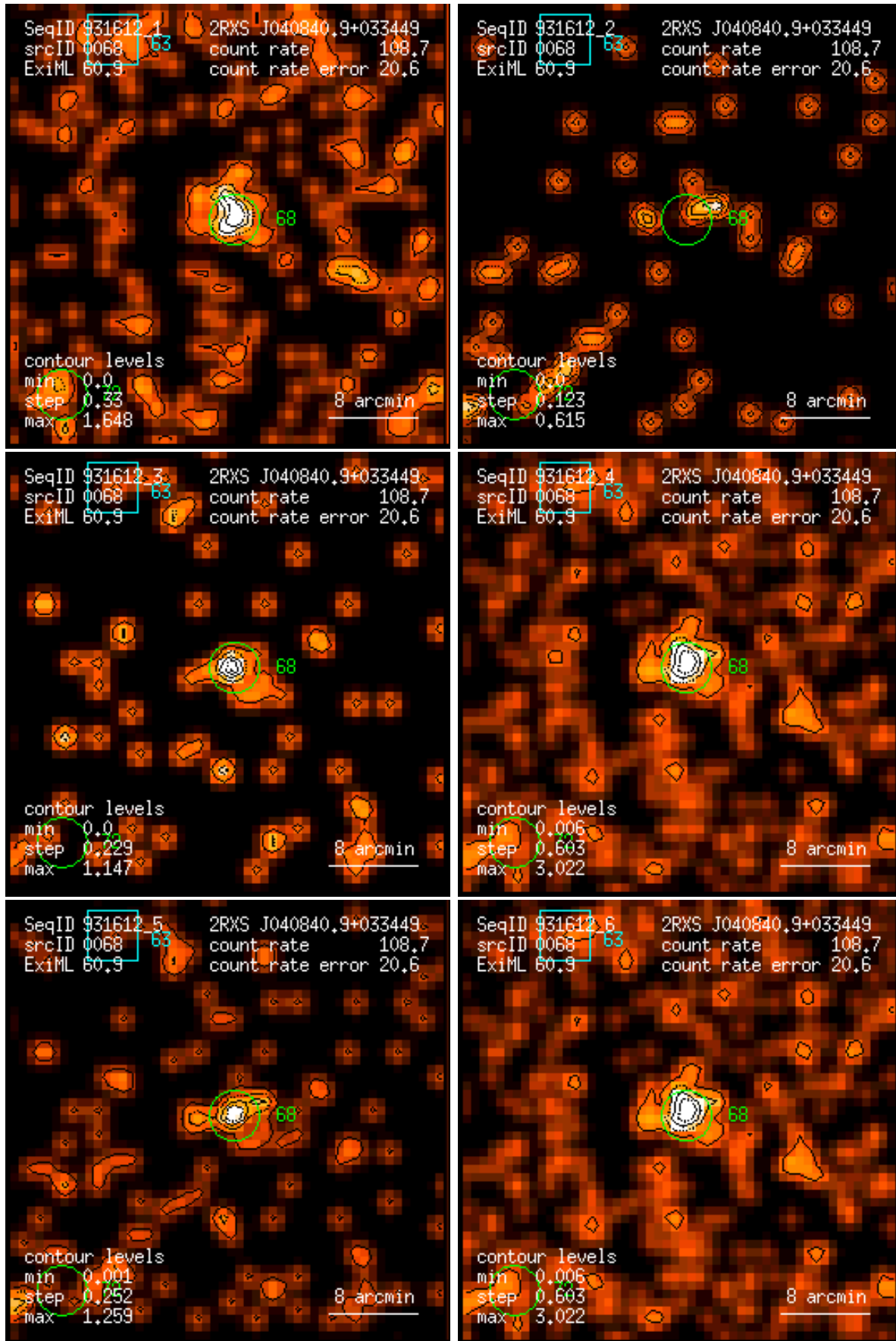
Figure 68: RASS 931612: detection 0068: band rate images, Gaussian filter: (1) PSPC channels 11 – 41, (2) 52 – 90, (3) 91 – 201, (4) 11 – 235, (5) 52 – 201, (6) 11 – 201. Broad band rates in counts/ks. Band rate contour levels in counts/ks/arcmin 2 .
