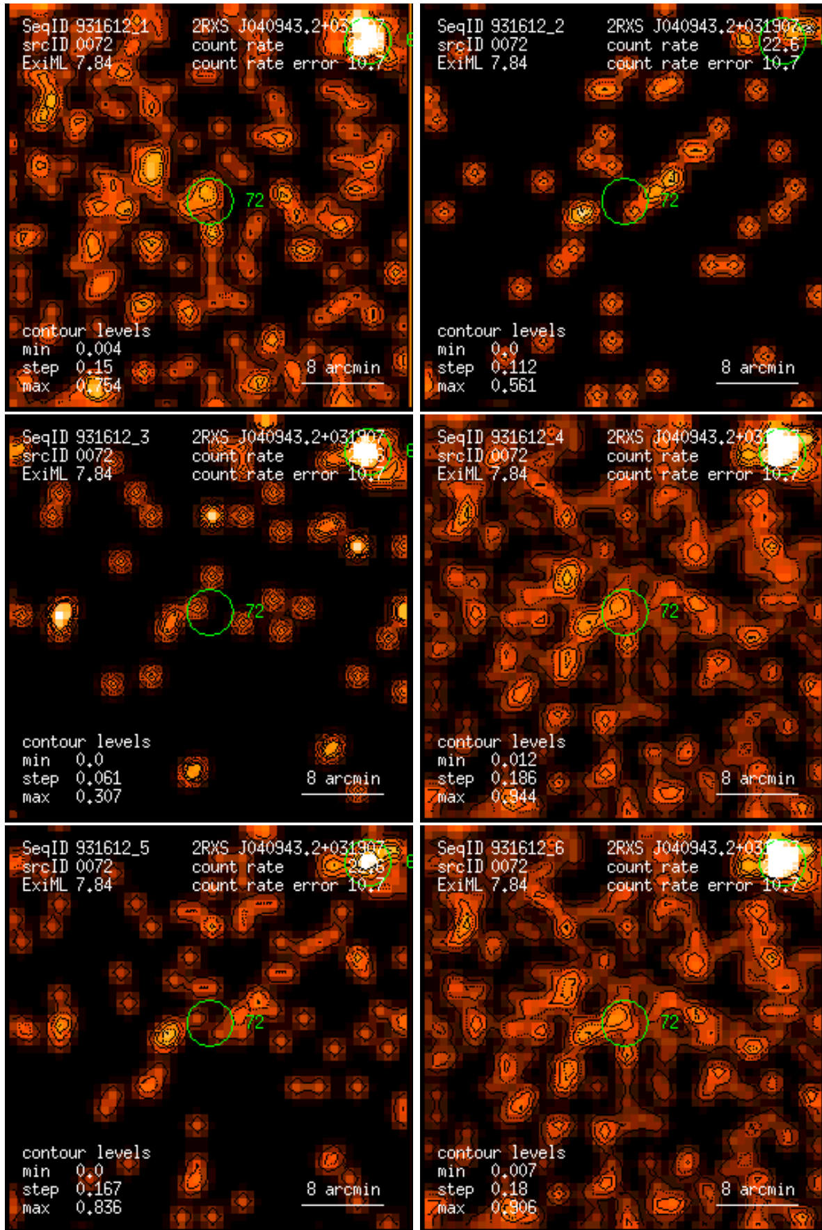
Figure 72: RASS 931612: detection 0072: band rate images, Gaussian filter: (1) PSPC channels 11 – 41, (2) 52 – 90, (3) 91 – 201, (4) 11 – 235, (5) 52 – 201, (6) 11 – 201. Broad band rates in counts/ks. Band rate contour levels in counts/ks/arcmin 2 .
