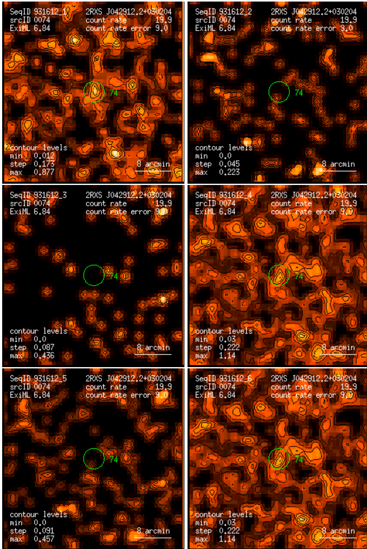
Figure 74: RASS 931612: detection 0074: band rate images, Gaussian filter: (1) PSPC channels 11 – 41, (2) 52 – 90, (3) 91 – 201, (4) 11 – 235, (5) 52 – 201, (6) 11 – 201. Broad band rates in counts/ks. Band rate contour levels in counts/ks/arcmin 2 .
