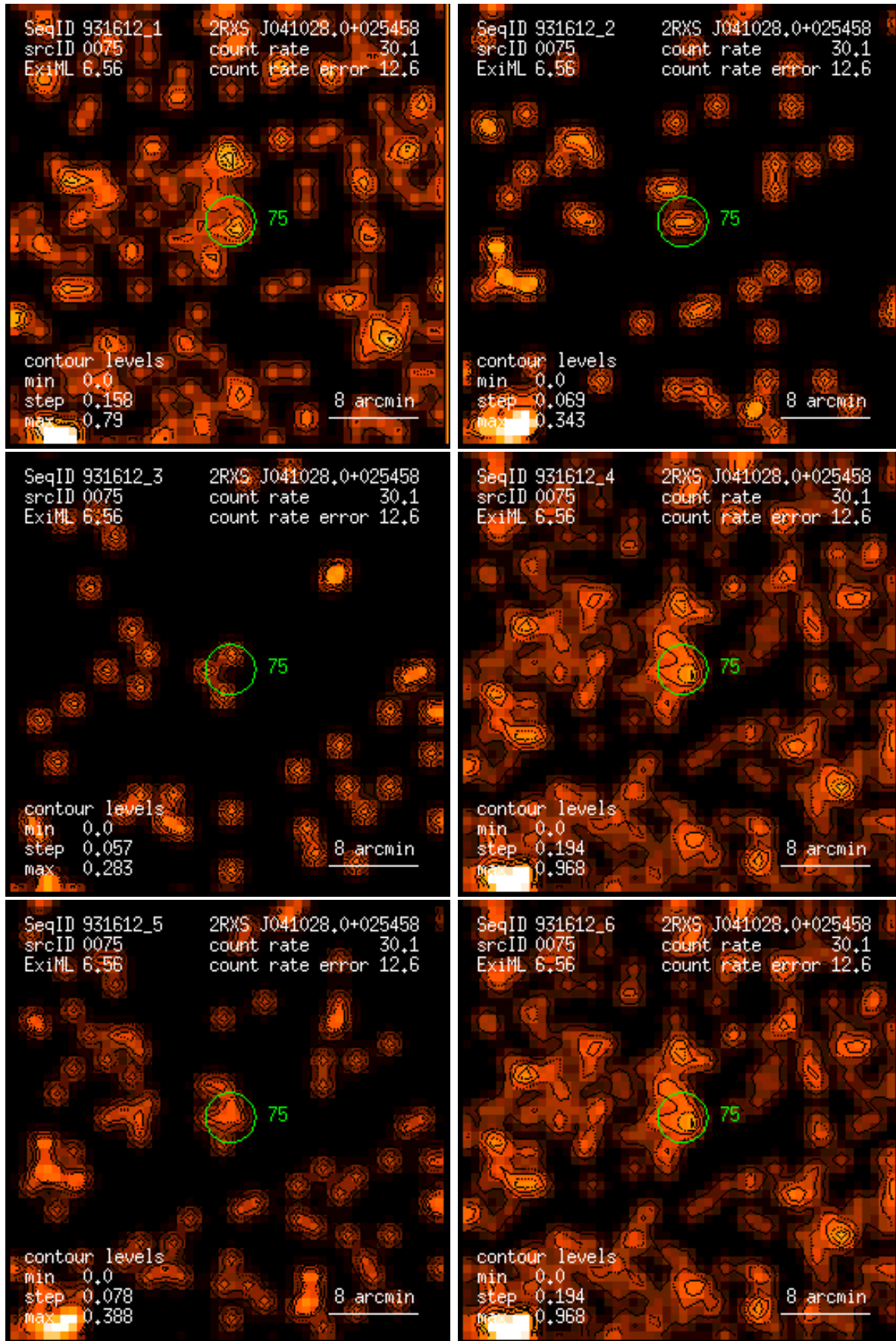
Figure 75: RASS 931612: detection 0075: band rate images, Gaussian filter: (1) PSPC channels 11 – 41, (2) 52 – 90, (3) 91 – 201, (4) 11 – 235, (5) 52 – 201, (6) 11 – 201. Broad band rates in counts/ks. Band rate contour levels in counts/ks/arcmin 2 .
