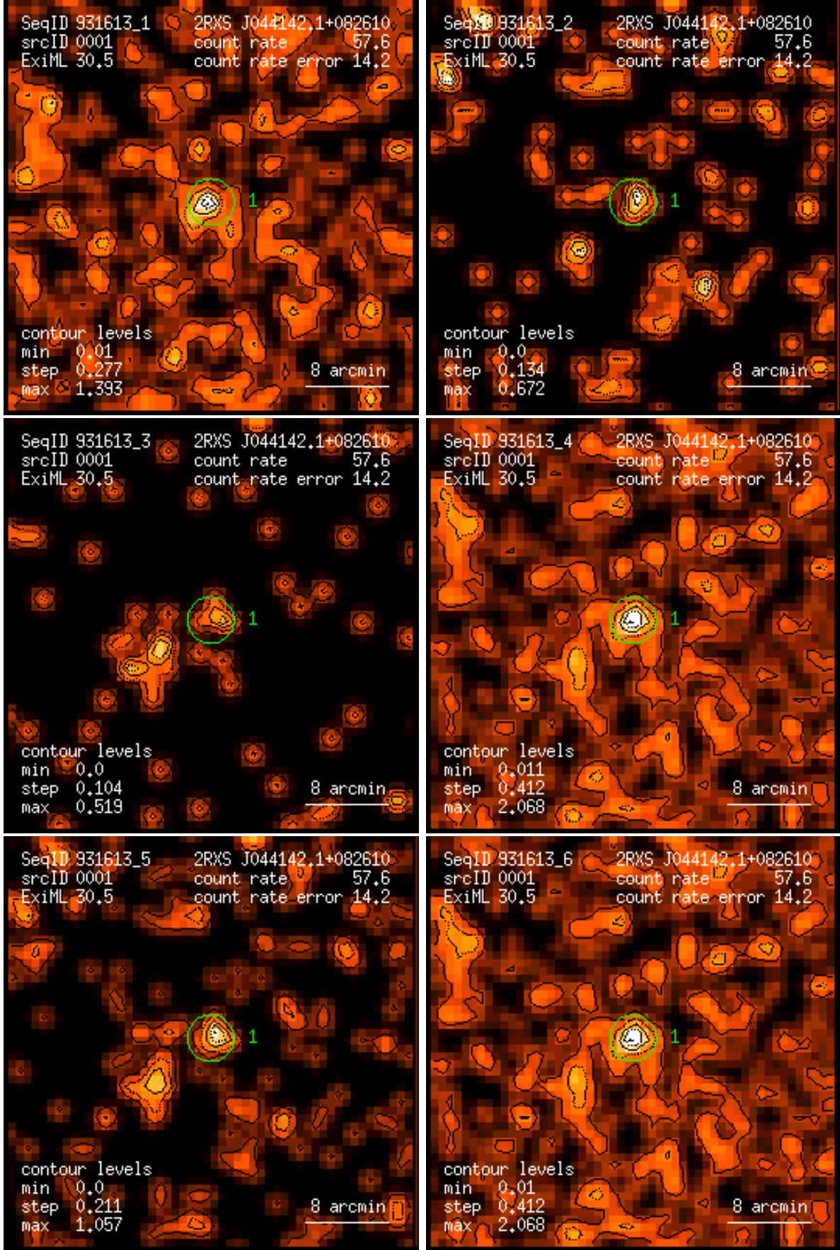
Figure 1: RASS 931613: detection 0001: band rate images, Gaussian filter: (1) PSPC channels 11 – 41, (2) 52 – 90, (3) 91 – 201, (4) 11 – 235, (5) 52 – 201, (6) 11 – 201. Broad band rates in counts/ks. Band rate contour levels in counts/ks/arcmin 2 .
