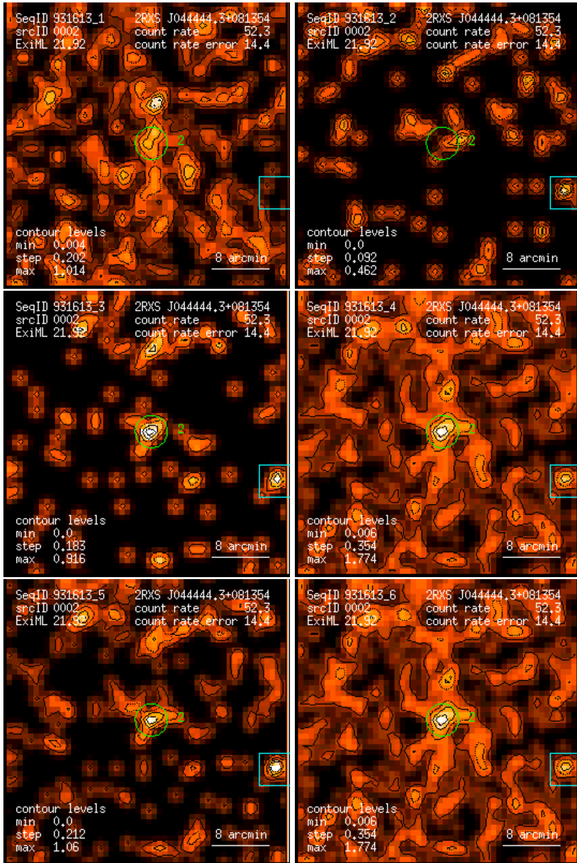
Figure 2: RASS 931613: detection 0002: band rate images, Gaussian filter: (1) PSPC channels 11 – 41, (2) 52 – 90, (3) 91 – 201, (4) 11 – 235, (5) 52 – 201, (6) 11 – 201. Broad band rates in counts/ks. Band rate contour levels in counts/ks/arcmin 2 .
