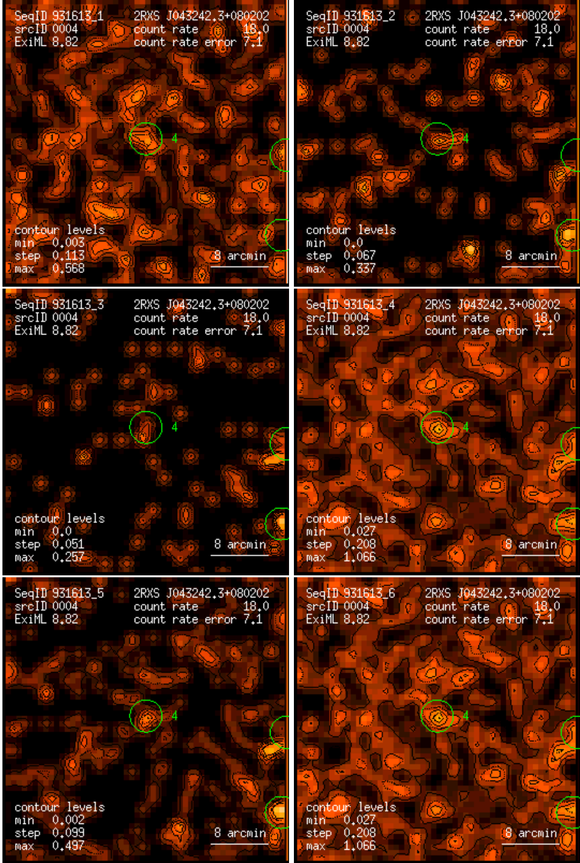
Figure 4: RASS 931613: detection 0004: band rate images, Gaussian filter: (1) PSPC channels 11 – 41, (2) 52 – 90, (3) 91 – 201, (4) 11 – 235, (5) 52 – 201, (6) 11 – 201. Broad band rates in counts/ks. Band rate contour levels in counts/ks/arcmin 2 .
